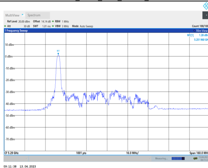
11AX80_Ant10_5290_52Tone_RU37
