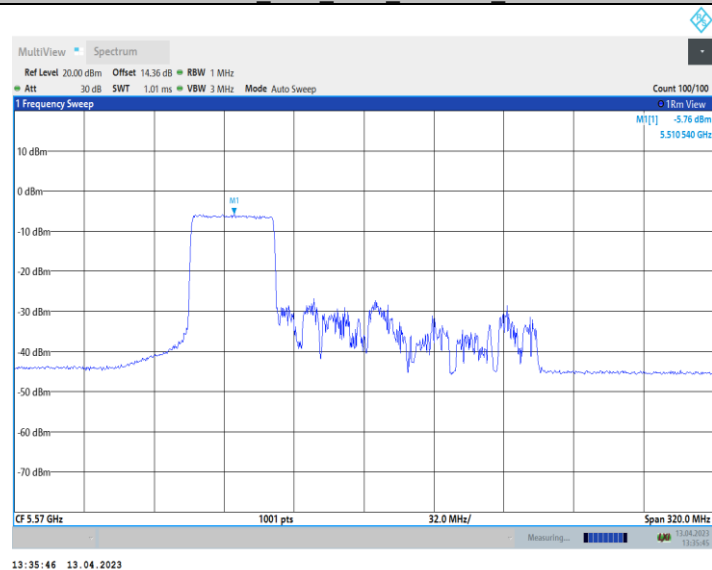
11AX160_Ant9_5570_996Tone_RU67
