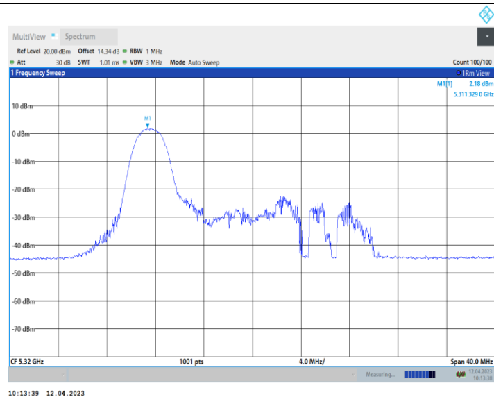
11AX20_Ant10_5320_52Tone_RU37
