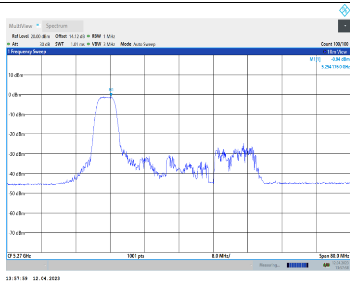
11AX40_Ant10_5270_106Tone_RU53
