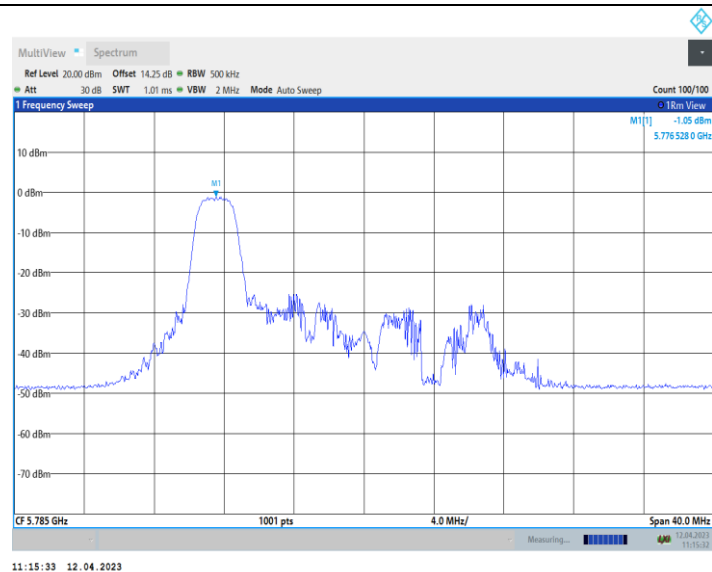
11AX20_Ant10_5785_52Tone_RU37
