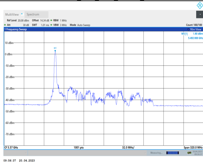
11AX160_Ant9_5570_52Tone_RU37
