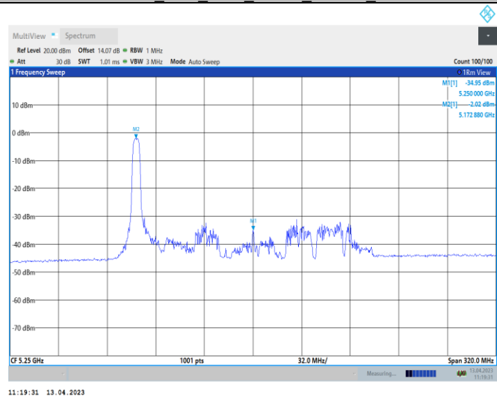
11AX160_Ant9_5250_UNII-1_106Tone_RU53
