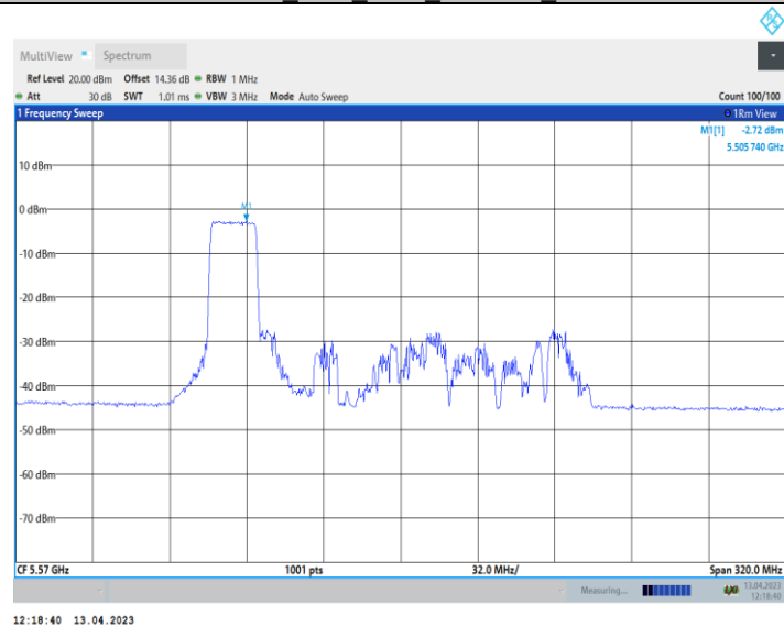
11AX160_Ant9_5570_484Tone_RU65
