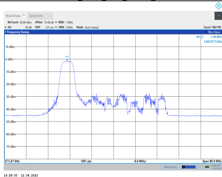
11AX40_Ant10_5670_106Tone_RU53
