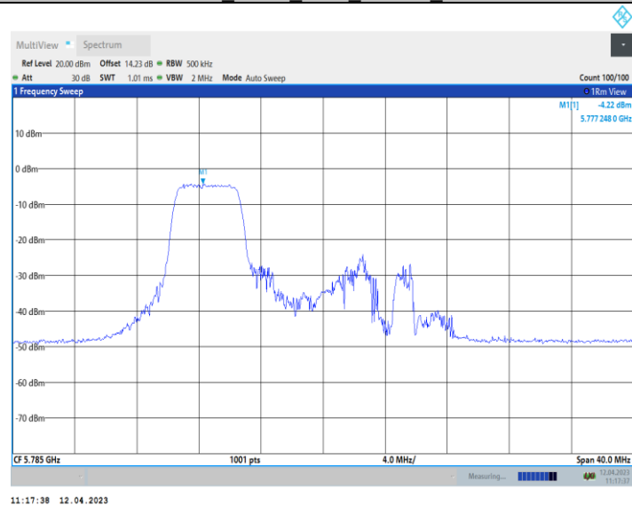
11AX20_Ant10_5785_106Tone_RU53
