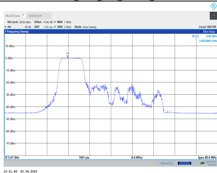
11AX40_Ant10_5670_242Tone_RU61
