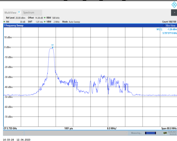
11AX40_Ant10_5755_52Tone_RU37
