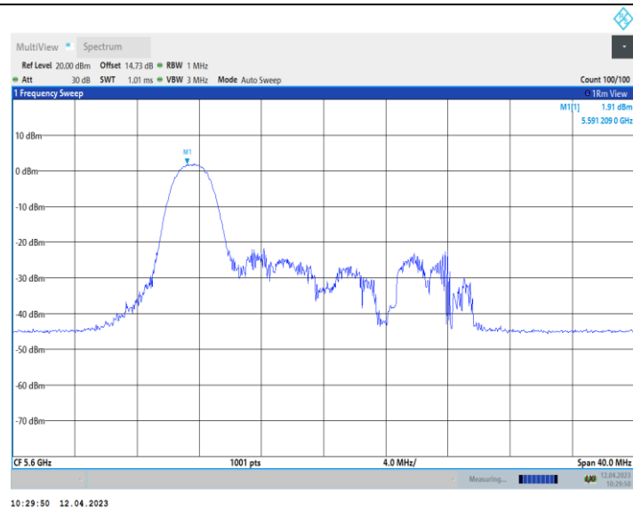
11AX20_Ant10_5600_52Tone_RU37
