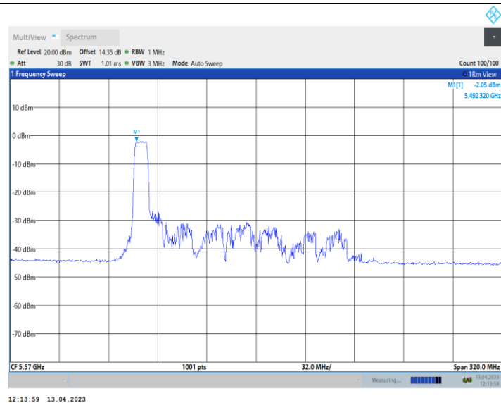
11AX160_Ant9_5570_242Tone_RU61
