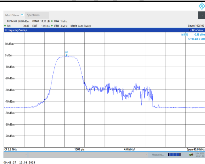
11AX20_Ant10_5200_106Tone_RU53
