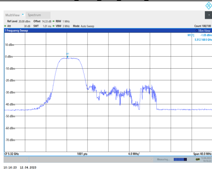
11AX20_Ant10_5320_106Tone_RU53
