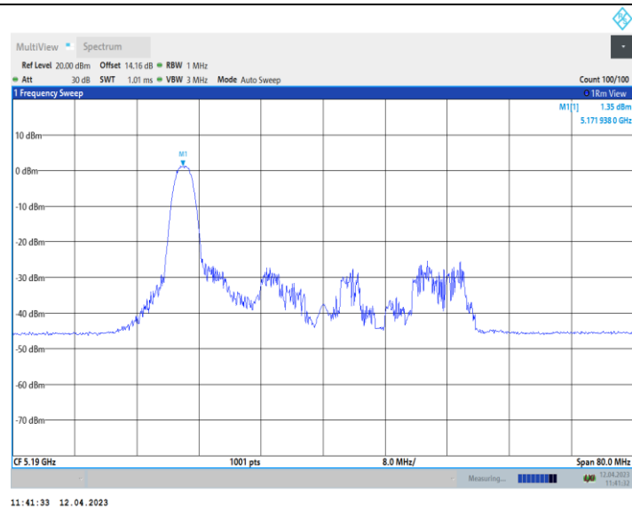
11AX40_Ant10_5190_52Tone_RU37
