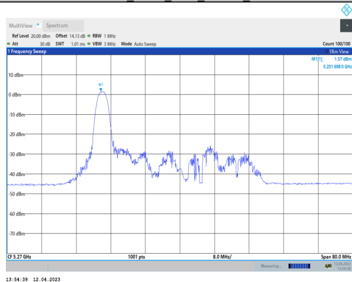
11AX40_Ant10_5270_52Tone_RU37
