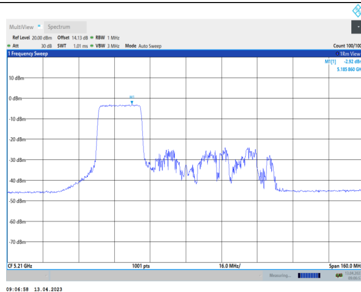
11AX80_Ant10_5210_484Tone_RU65
