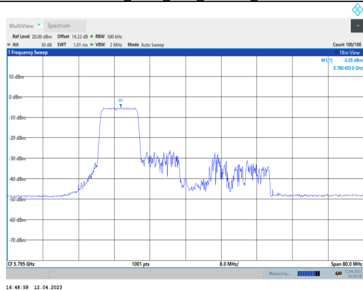
11AX40_Ant10_5795_242Tone_RU61
