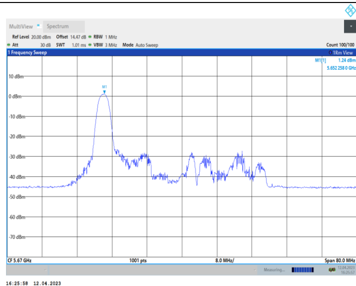
11AX40_Ant10_5670_52Tone_RU37
