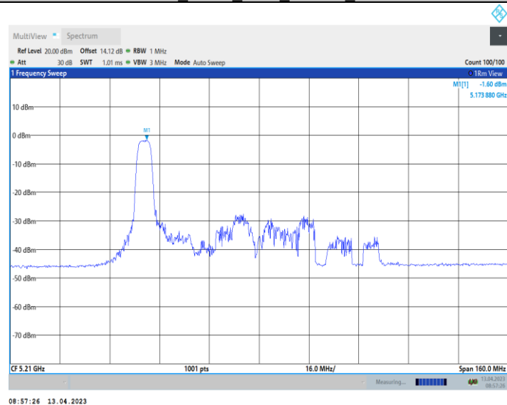
11AX80_Ant10_5210_106Tone_RU53
