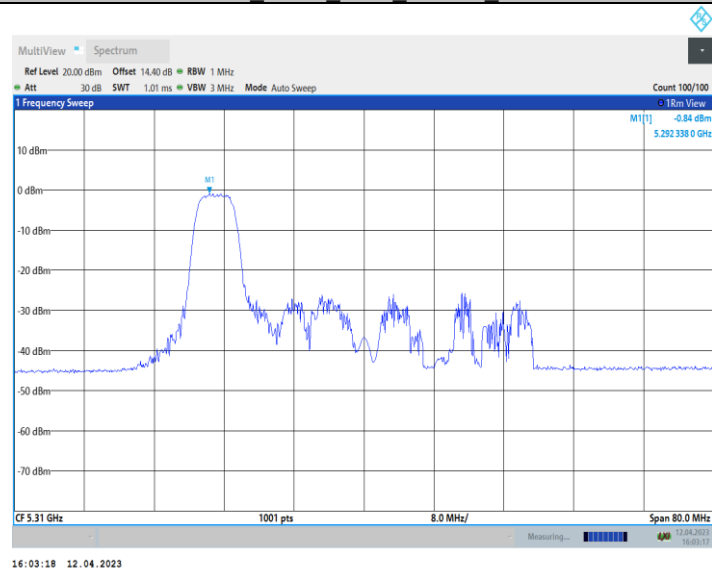
11AX40_Ant10_5310_106Tone_RU53
