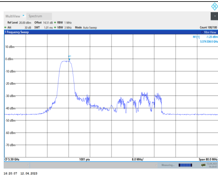
11AX40_Ant10_5590_106Tone_RU53
