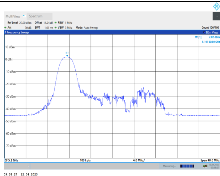
11AX20_Ant10_5200_52Tone_RU37
