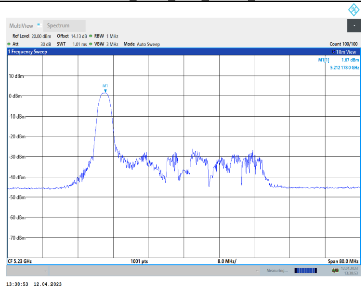
11AX40_Ant10_5230_52Tone_RU37
