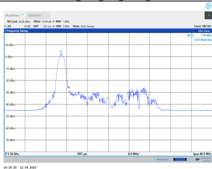
11AX40_Ant10_5590_52Tone_RU37
