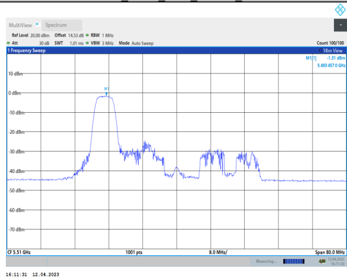
11AX40_Ant10_5510_106Tone_RU53
