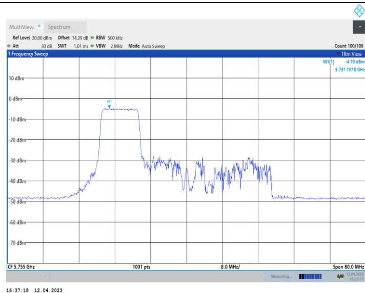
11AX40_Ant10_5755_242Tone_RU61
