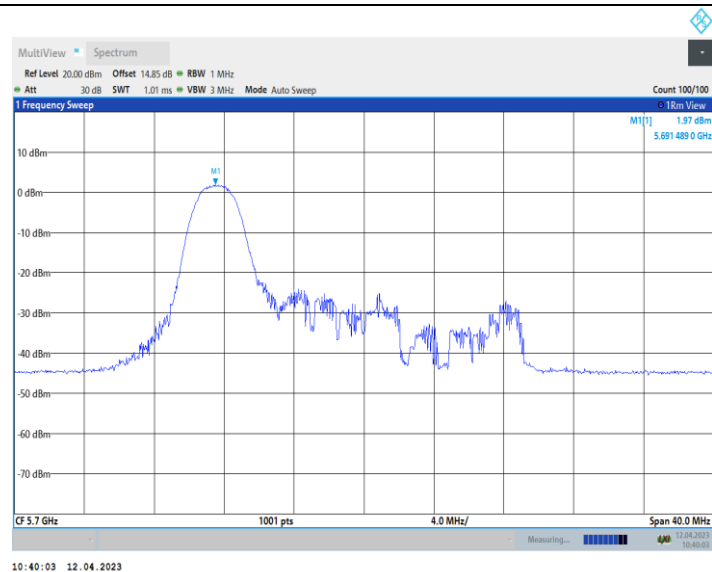
11AX20_Ant10_5700_52Tone_RU37
