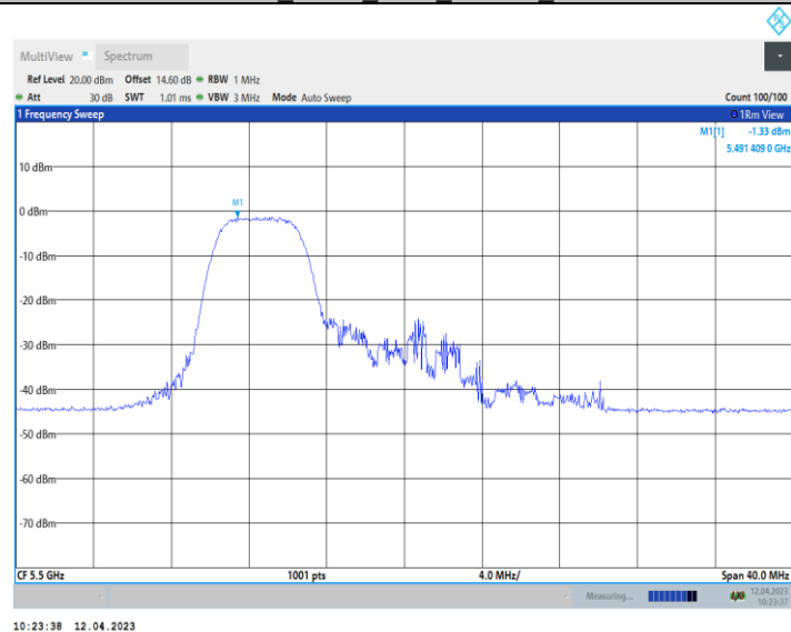
11AX20_Ant10_5500_106Tone_RU53
