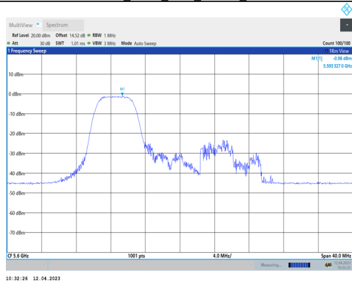
11AX20_Ant10_5600_106Tone_RU53
