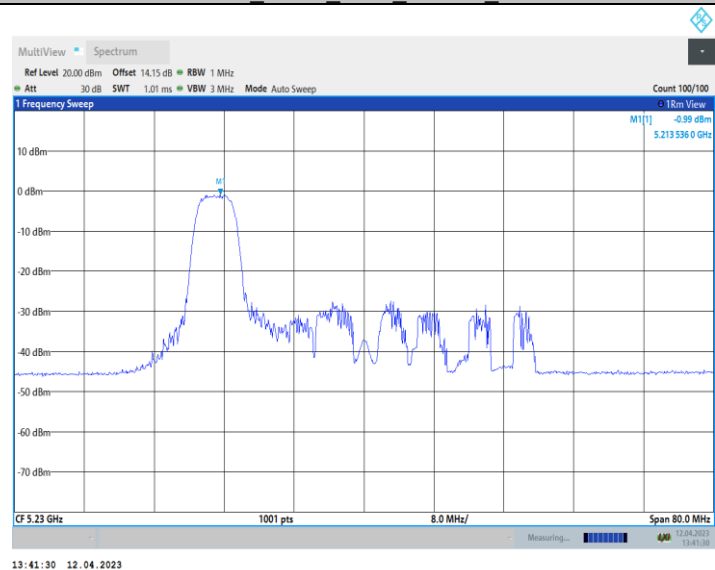
11AX40_Ant10_5230_106Tone_RU53
