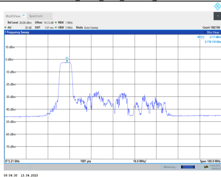
11AX80_Ant10_5210_242Tone_RU61
