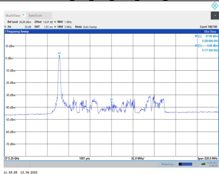
11AX160_Ant9_5250_UNII-1_52Tone_RU37
