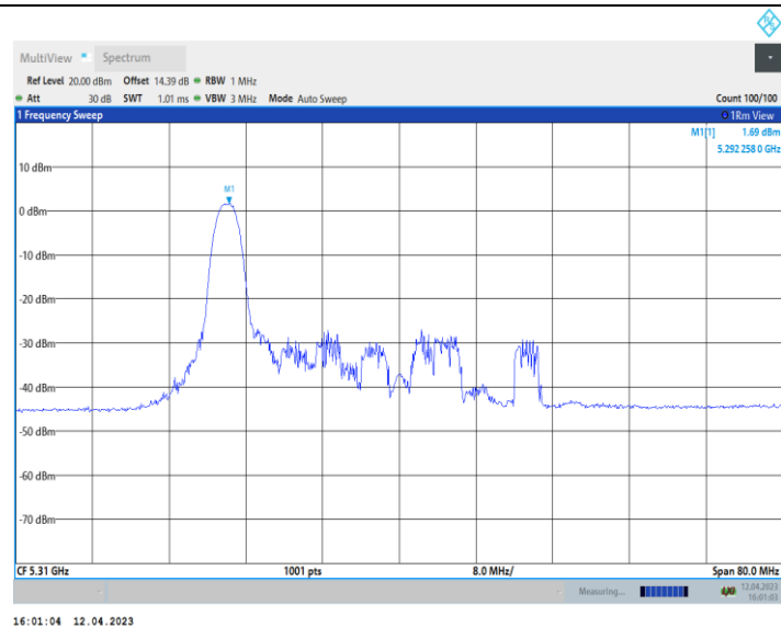
11AX40_Ant10_5310_52Tone_RU37
