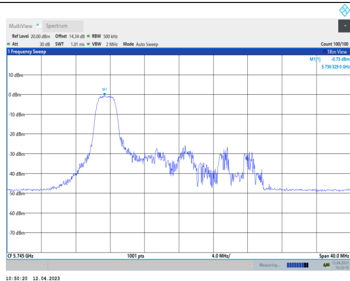
11AX20_Ant10_5745_52Tone_RU37
