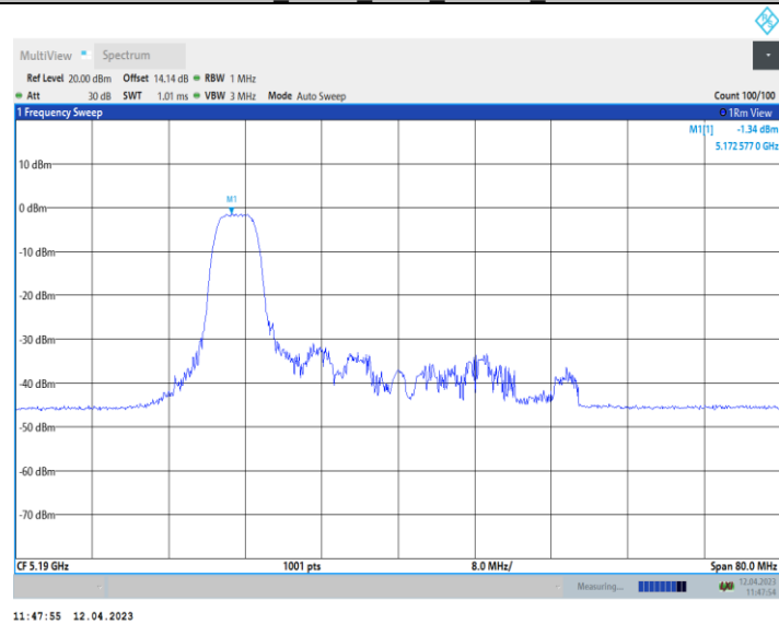
11AX40_Ant10_5190_106Tone_RU53
