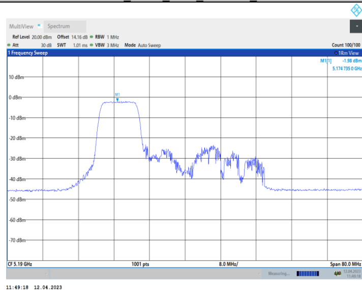
11AX40_Ant10_5190_242Tone_RU61
