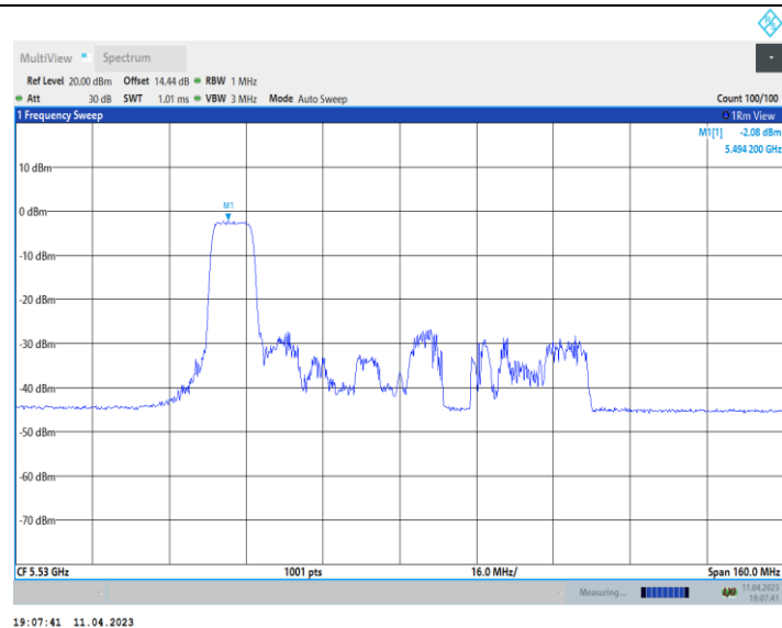
11AX80_Ant9_5530_242Tone_RU61
