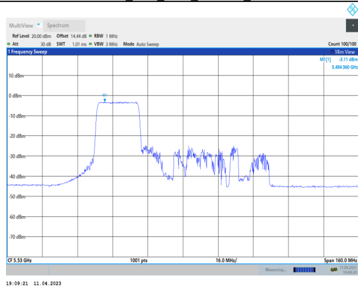
11AX80_Ant9_5530_484Tone_RU65
