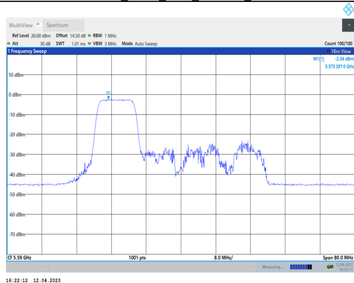
11AX40_Ant10_5590_242Tone_RU61
