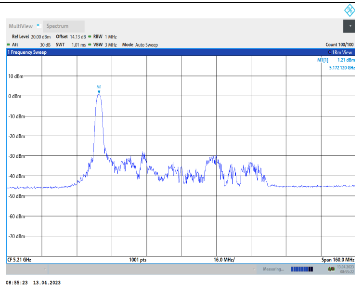
11AX80_Ant10_5210_52Tone_RU37
