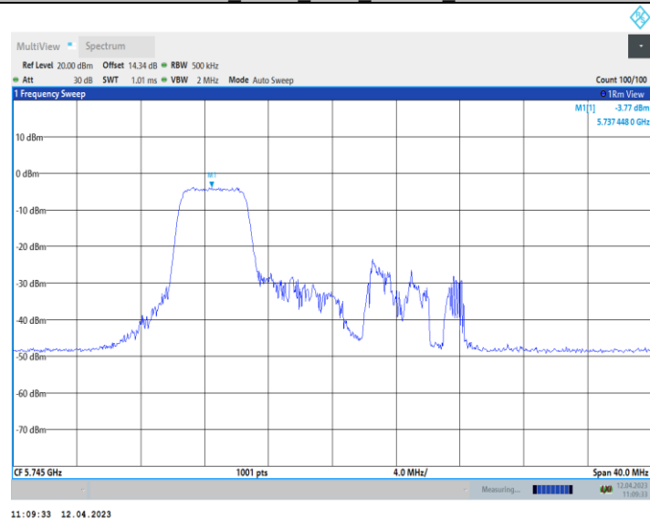
11AX20_Ant10_5745_106Tone_RU53
