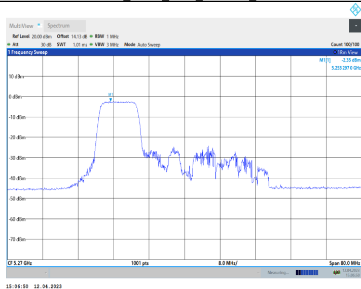
11AX40_Ant10_5270_242Tone_RU61
