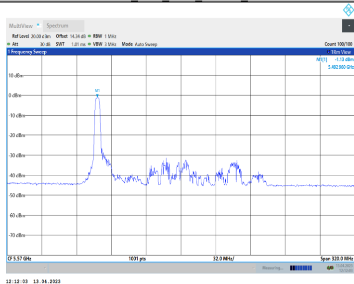
11AX160_Ant9_5570_106Tone_RU53
