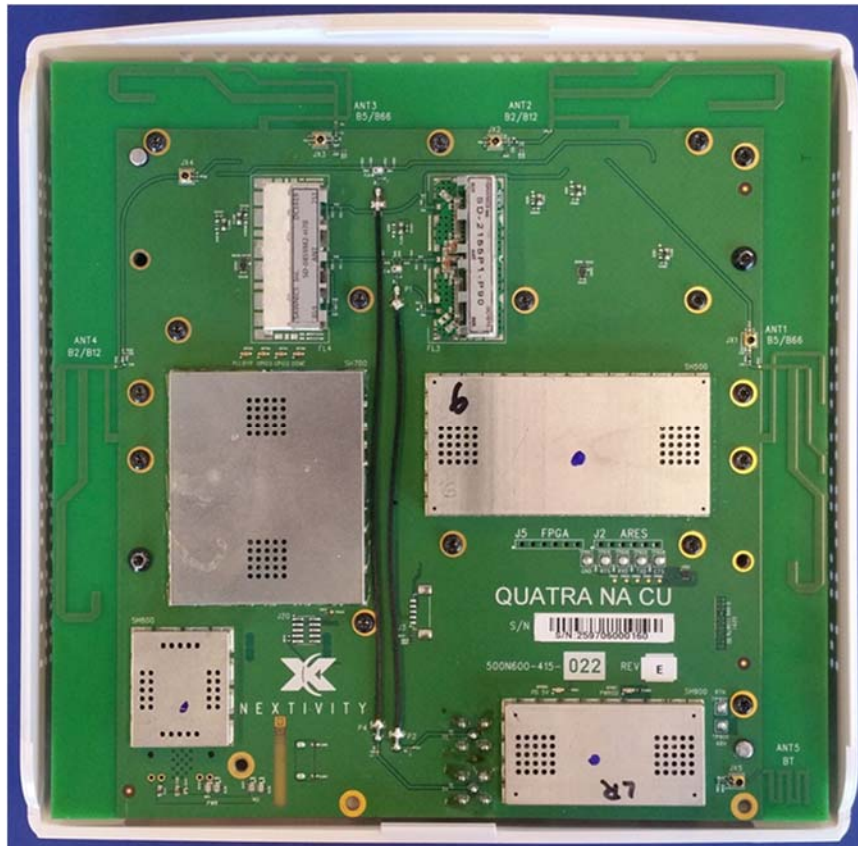
Housing_1 / PCB_side 1
