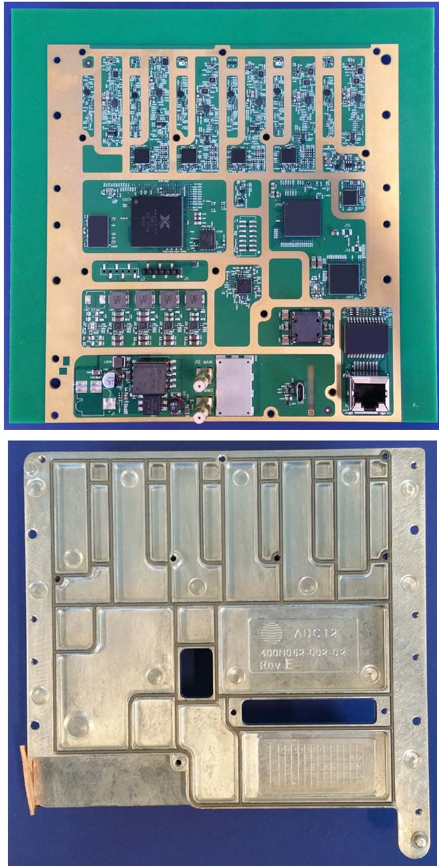
Heatsink / PCB Side 2
