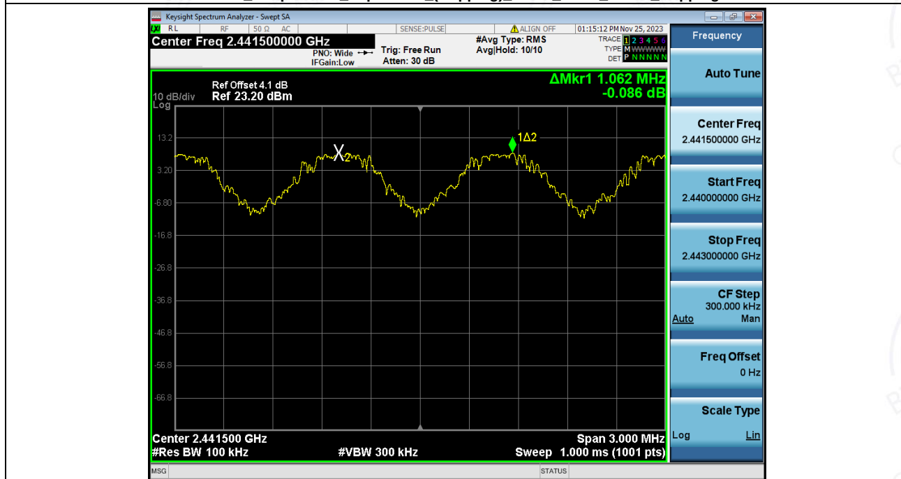
Carrier_Frequencies_Separation_(Hopping)_NVNT_ANT1_1-DH5_Hopping
