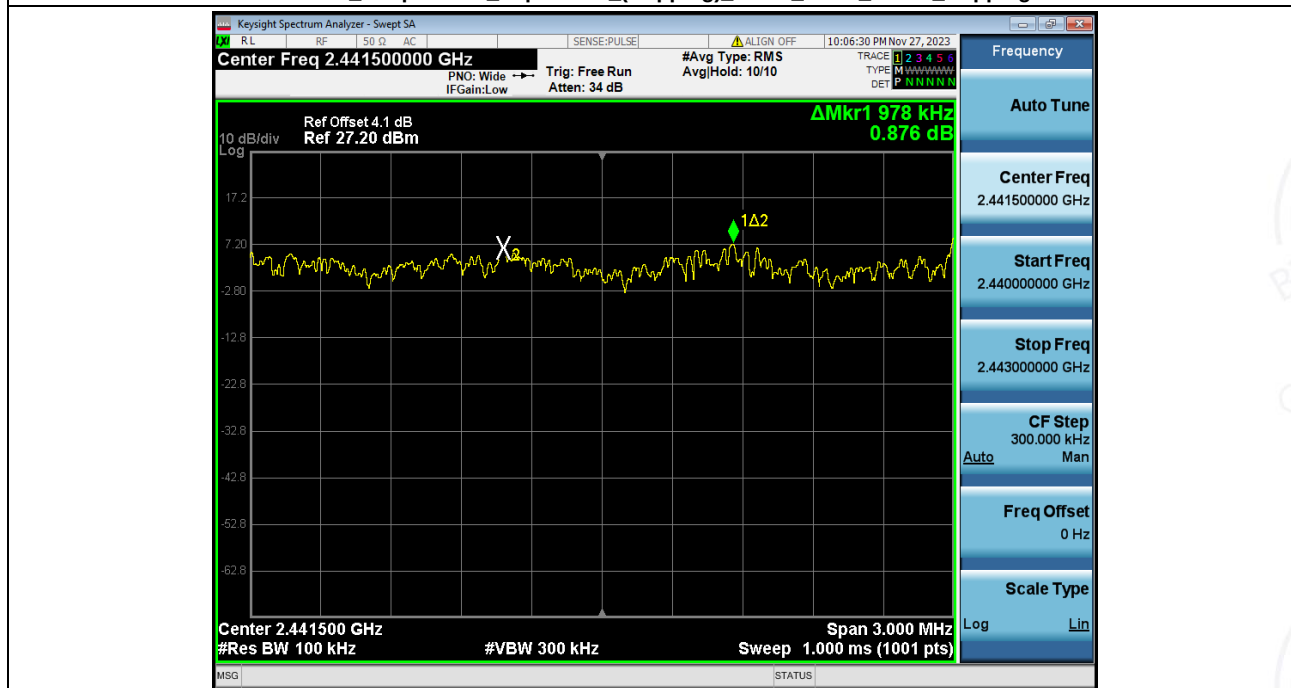
Carrier_Frequencies_Separation_(Hopping)_NVNT_ANT1_2-DH5_Hopping
