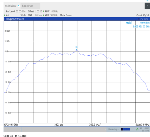
BLE_2M-Ant6-2404-0~Reference-PASS
