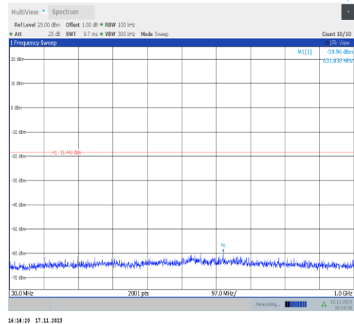
BLE_1M-Ant6-2480-30~1000-PASS
