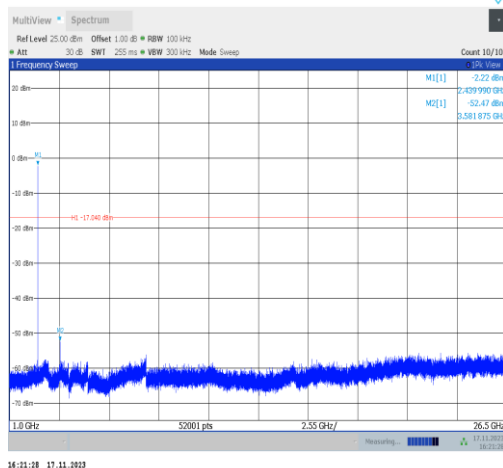
BLE_2M-Ant6-2440-1000~26500-PASS
