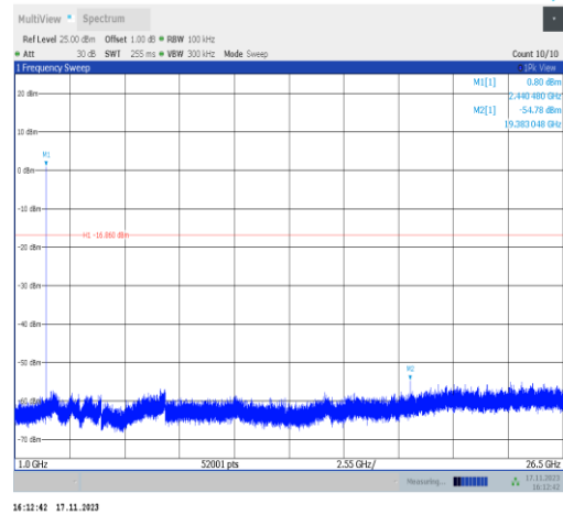
BLE_1M-Ant6-2440-1000~26500-PASS
