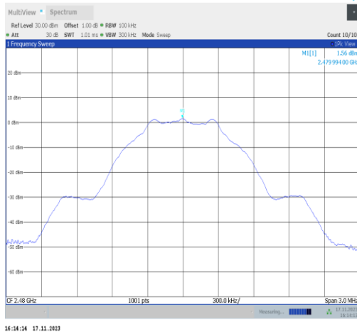
BLE_1M-Ant6-2480-0~Reference-PASS
