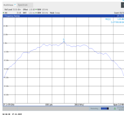
BLE_2M-Ant6-2478-0~Reference-PASS
