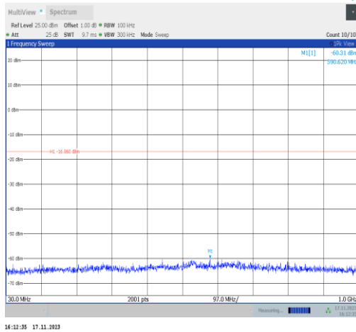
BLE_1M-Ant6-2440-30~1000-PASS
