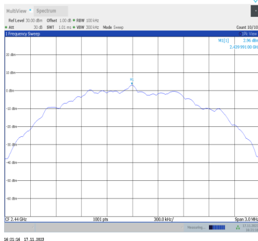
BLE_2M-Ant6-2440-0~Reference-PASS
