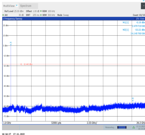
BLE_1M-Ant6-2480-1000~26500-PASS
