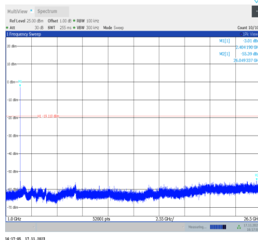
BLE_2M-Ant6-2404-1000~26500-PASS
