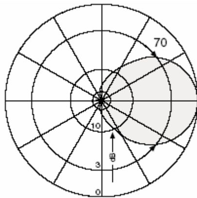
Horizontal pattern
