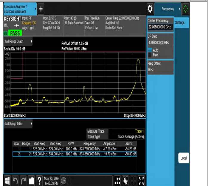
Band5_10MHz_QPSK_20450_1RB#49
