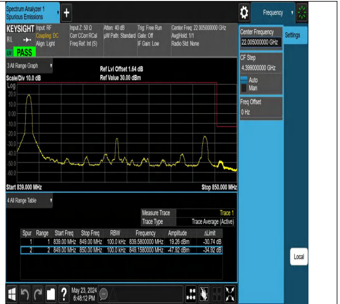
Band5_10MHz_QPSK_20600_1RB#0
