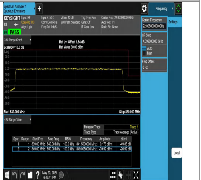
Band5_10MHz_QPSK_20600_50RB#0
