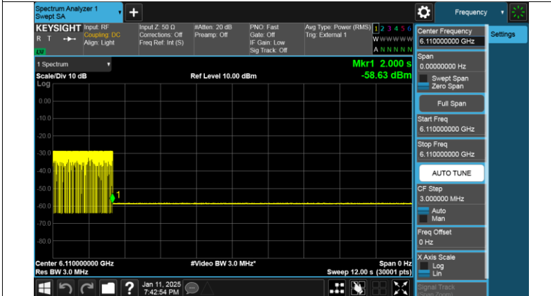
Contention Based Protocol NVNT be160 6185MHz Interfere 6110 MHz_8
