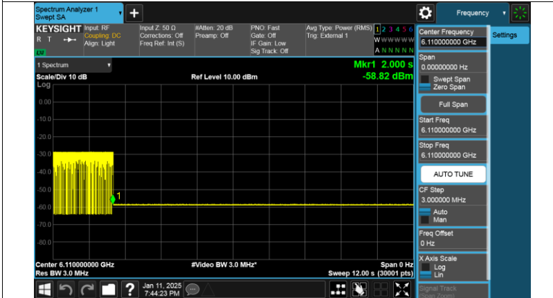
Contention Based Protocol NVNT be160 6185MHz Interfere 6110 MHz_7
