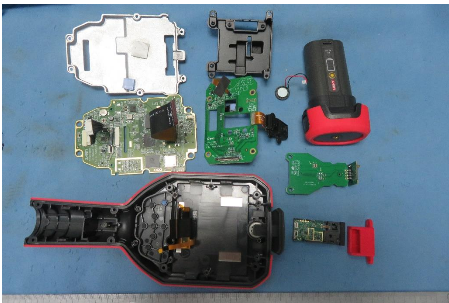
Internal view of model UTi720V, UTi720E
