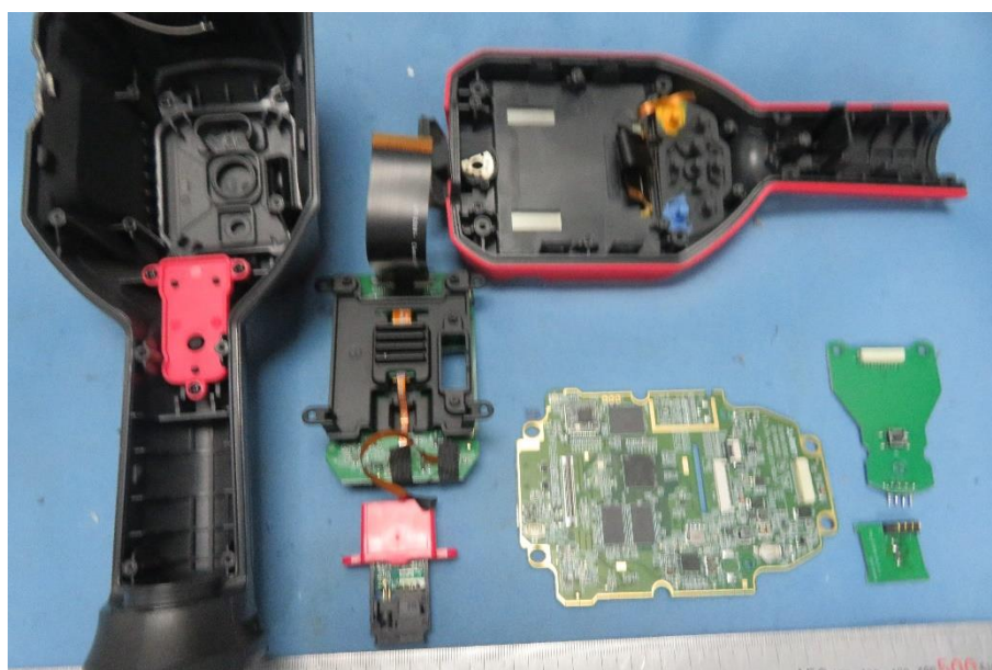
Internal view of model UTi730V, UTi730E
