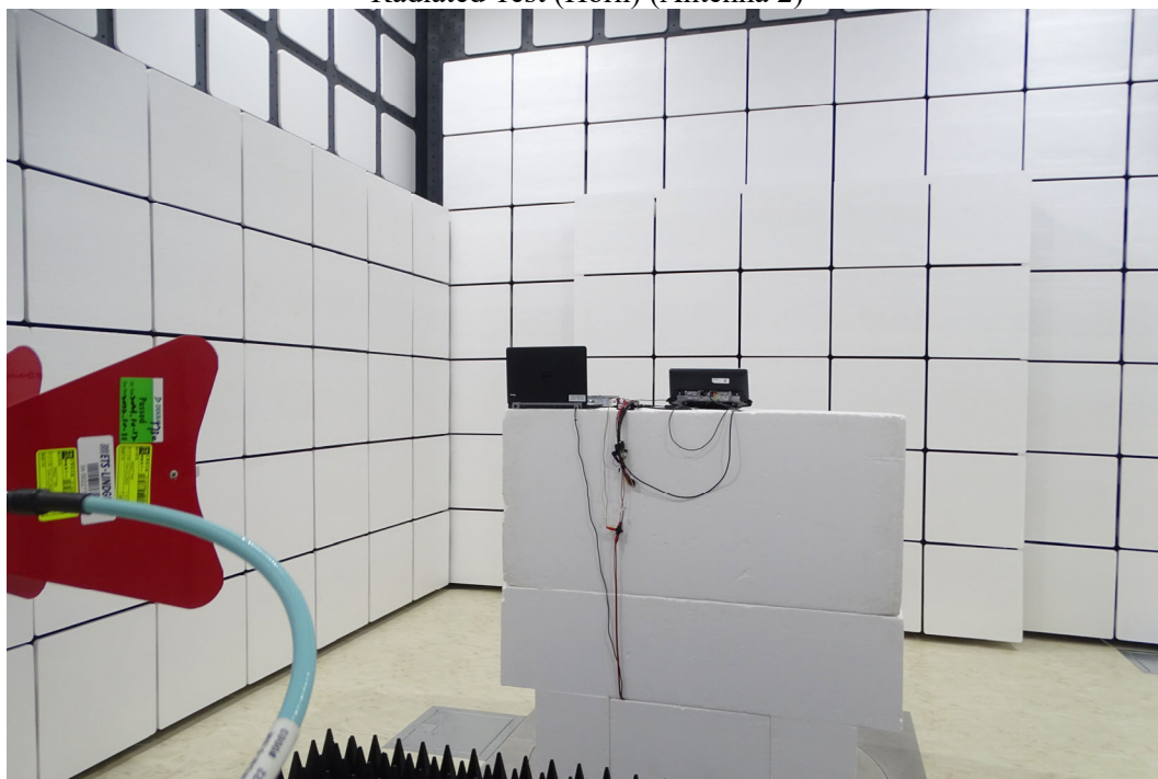
Radiated Test (Horn) (Antenna 2)
