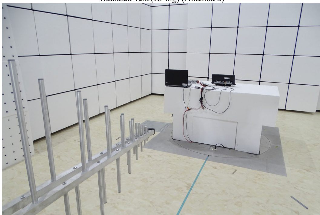
Radiated Test (Bi-log) (Antenna 2)
