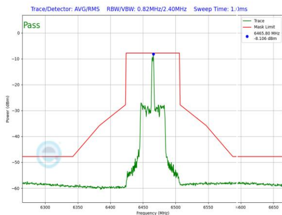
Plot 7-1114. LPI In-Band Emission Plot Antenna WF5B (80MHz 802.11ax RU26 (UNII Band 6) – Ch. 103)
