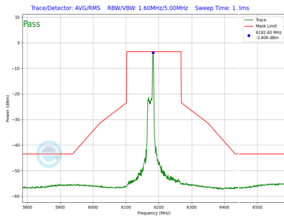
Plot 7-1166. LPI In-Band Emission Plot Antenna WF8 (160MHz 802.11ax RU26 (UNII Band 5) – Ch. 47)
