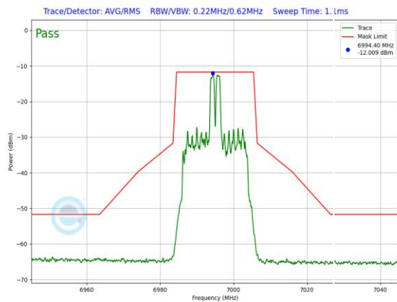
Plot 7-1138. LPI In-Band Emission Plot Antenna WF5B (20MHz 802.11ax RU26 (UNII Band 8) – Ch. 209)
