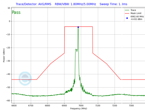
Plot 7-1150. LPI In-Band Emission Plot Antenna WF5B (160MHz 802.11ax RU26 (UNII Band 8) – Ch. 207)
