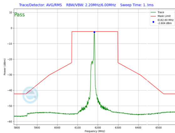
Plot 7-1102. LPI In-Band Emission Plot Antenna WF5B (160MHz 802.11ax RU26 (UNII Band 5) – Ch. 47)
