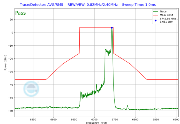
Plot 7-1077. SP In-Band Emission Plot CDD Diversity Antenna WF8 (80MHz 802.11ax RU26 (UNII Band 7) - Ch. 151)
