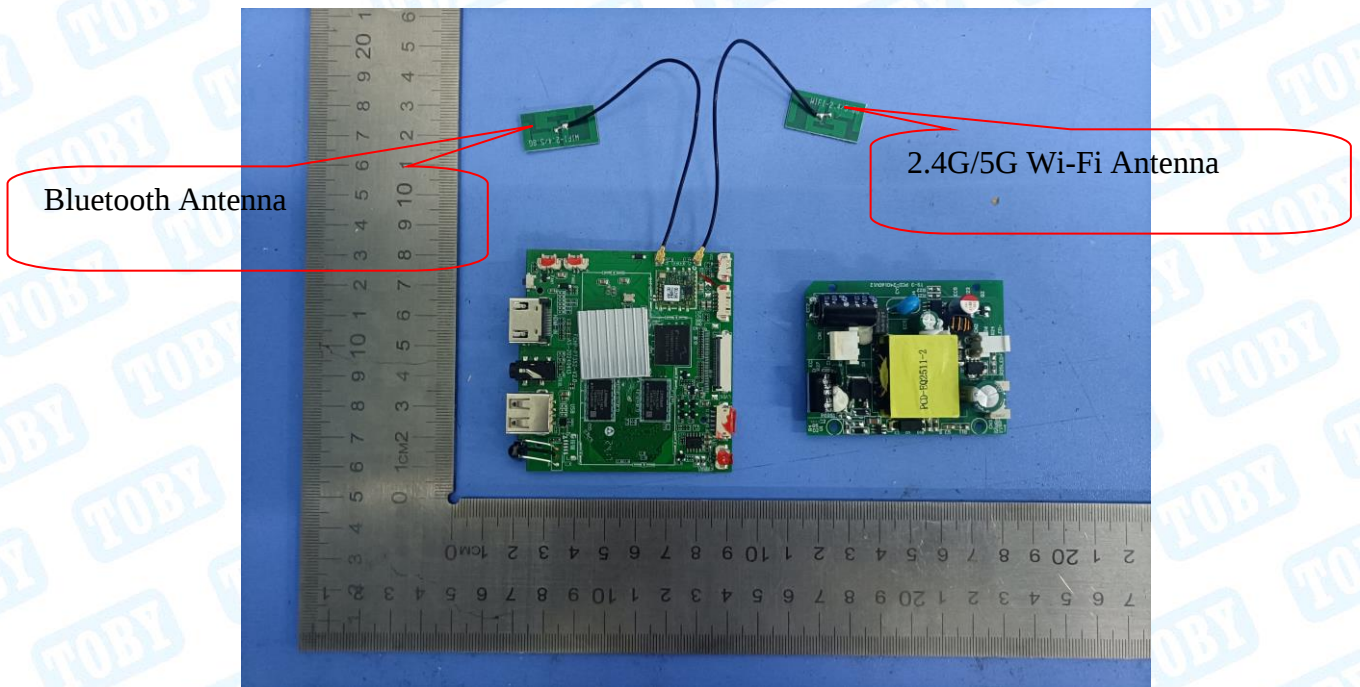
Photo 16 Appearance of PCB
