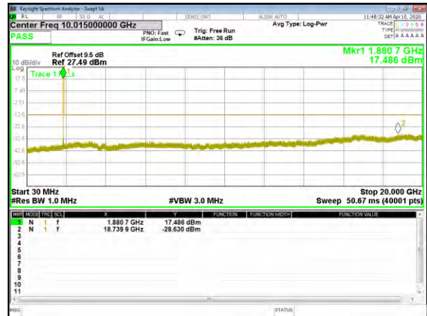
HSUPA B2_Conducted Spurious_Middle
