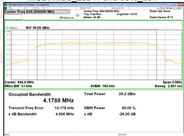
HSDPA B5_26BW and 99%_High
