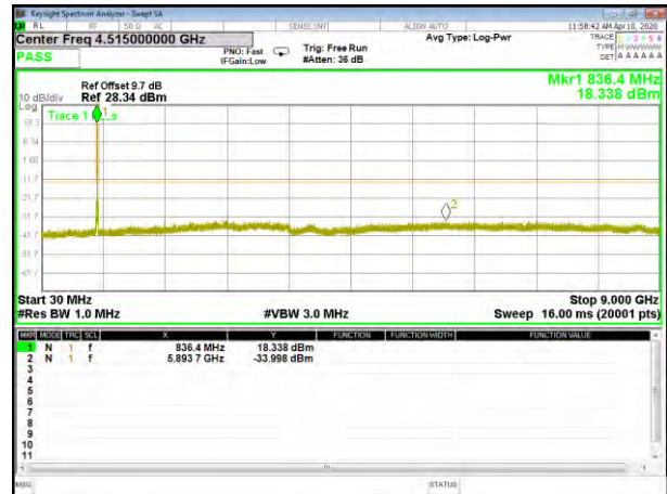
HSUPA B5_Conducted Spurious_Middle
