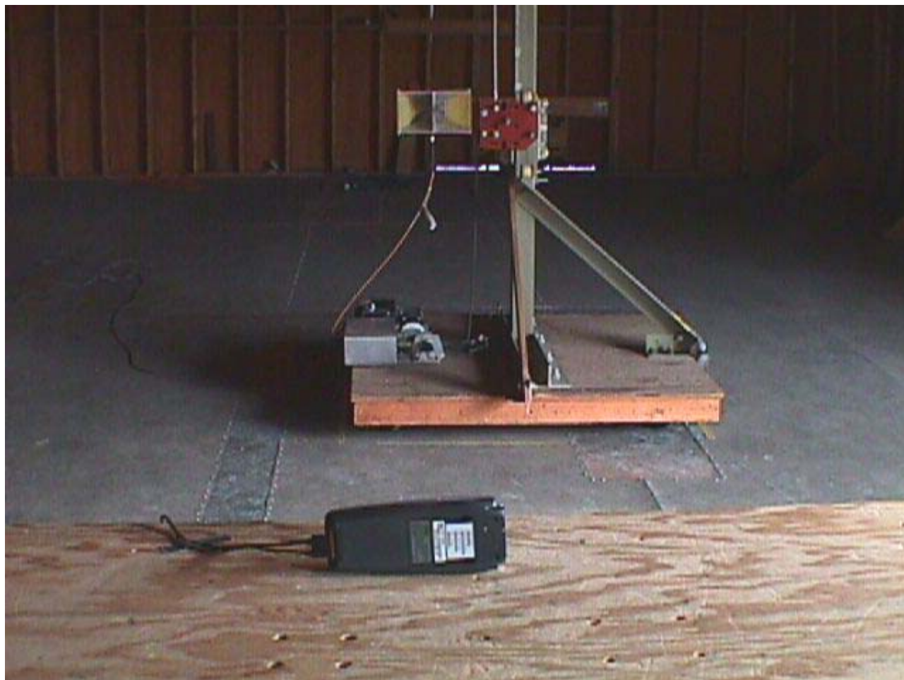
Radiated Emissions at 3 Meters Distance Orthogonal Position # 2
