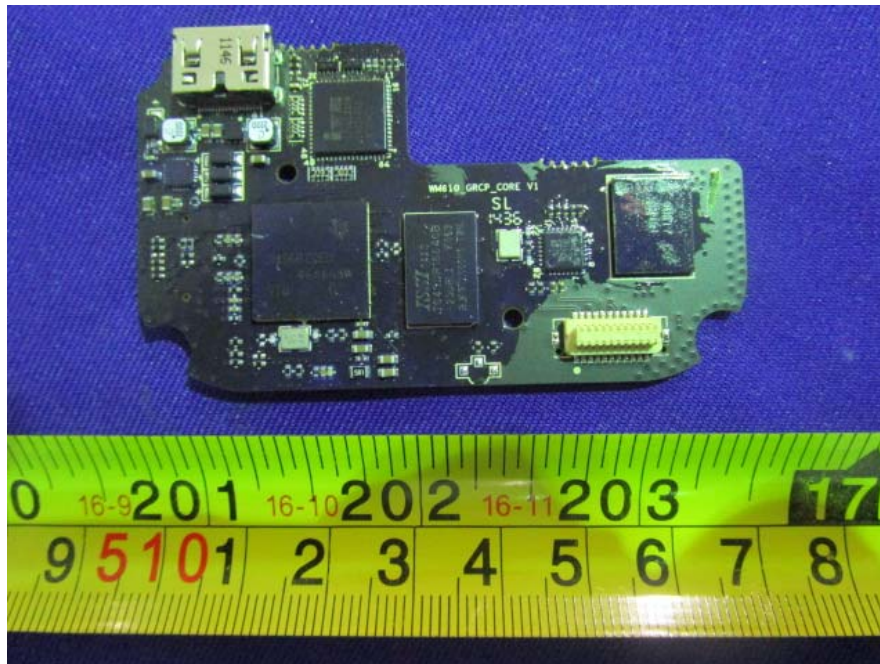
EUT – HDMI Board Top View
