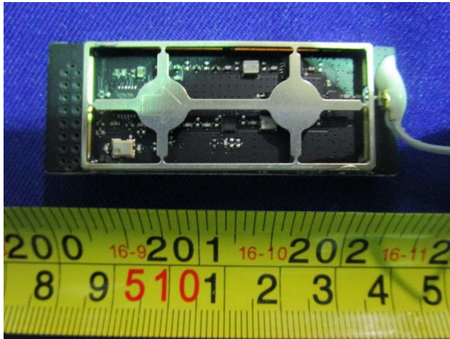
EUT – 5.8GHz RF Module Top without ShieldingView
