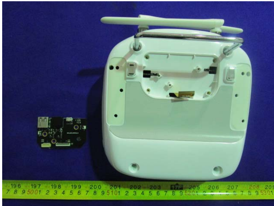
EUT – Port Board Off View
