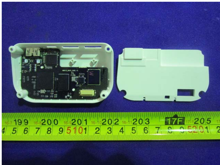
EUT – HDMI Box Uncover View
