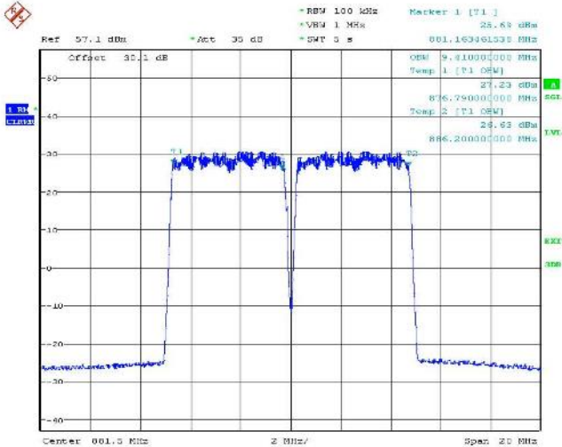
Figure 105 Occupied Bandwidth – QPSK (879/884 MHz) (5+5MHz Channel BW)
