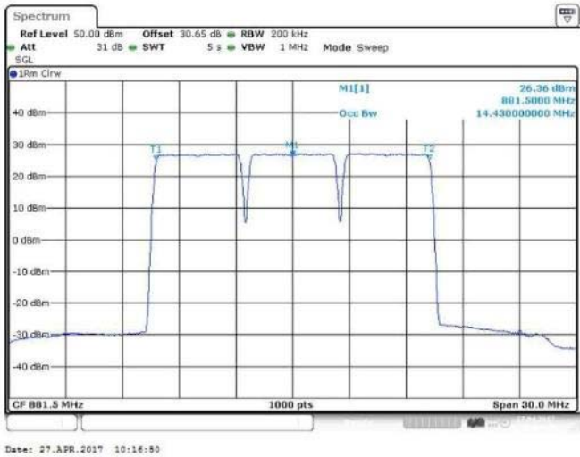
Figure 55 Occupied Bandwidth – 64QAM (876.5, 881.5, 886.5 MHz) (3 X 5 MHz Channel BW)
