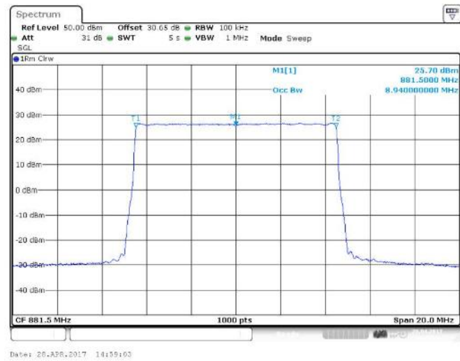
Figure 76 Occupied Bandwidth – 256QAM (881.5 MHz) (1 X 10 MHz Channel BW)
