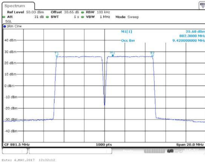
Figure 40 Occupied Bandwidth – 256QAM (879 MHz, 884 MHz) (2 X 5 MHz Channel BW)
