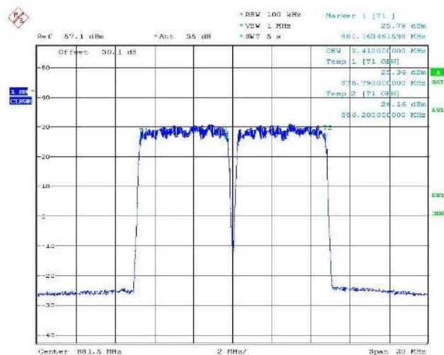
Figure 101 Occupied Bandwidth – QPSK (879/884 MHz) (5+5MHz Channel BW)
