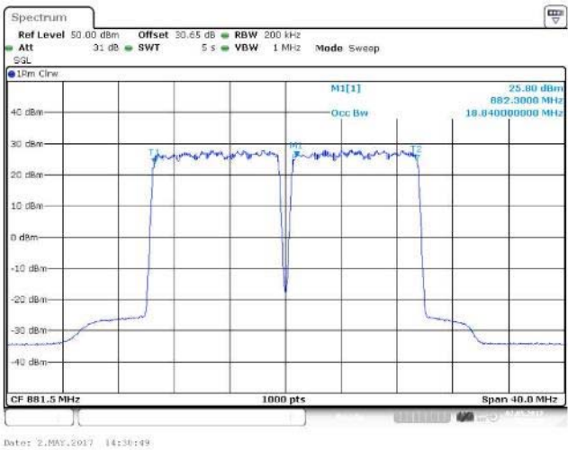
Figure 82 Occupied Bandwidth – 16QAM (876.5 MHz, 886.5 MHz) (2 X 10 MHz Channel BW)
