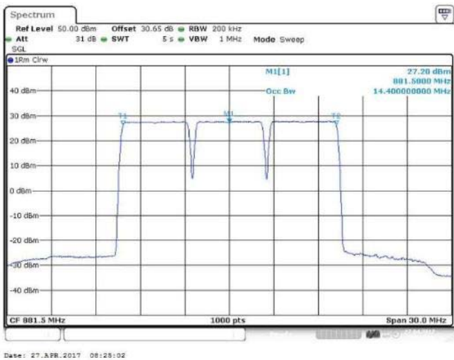
Figure 47 Occupied Bandwidth – 64QAM (876.5, 881.5, 886.5 MHz) (3 X 5 MHz Channel BW)
