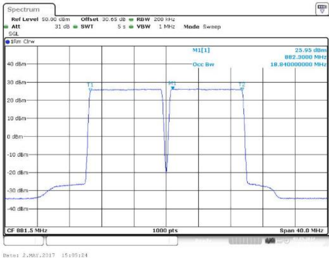
Figure 84 Occupied Bandwidth – 256QAM (876.5 MHz, 886.5 MHz) (2 X 10 MHz Channel BW)
