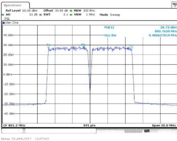
Figure 38 Occupied Bandwidth – 16QAM (879 MHz, 884 MHz) (2 X 5 MHz Channel BW)
