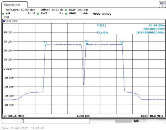
Figure 79 Occupied Bandwidth – 64QAM (876.5 MHz, 886.5 MHz) (2 X 10 MHz Channel BW)
