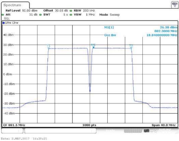
Figure 85 Occupied Bandwidth – QPSK (876.5 MHz, 886.5 MHz) (2 X 10 MHz Channel BW)
