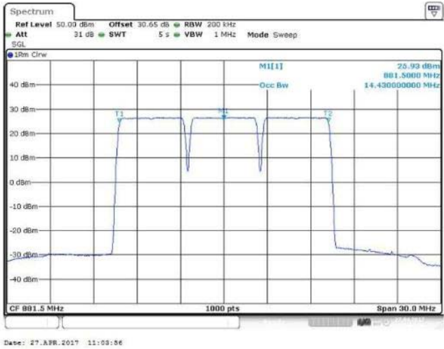
Figure 56 Occupied Bandwidth – 256QAM (876.5, 881.5, 886.5 MHz) (3 X 5 MHz Channel BW)
