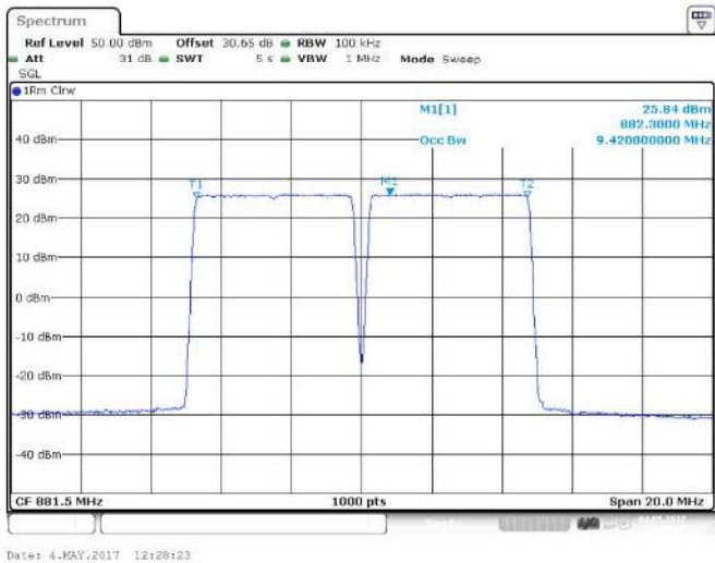
Figure 36 Occupied Bandwidth – 256QAM (879 MHz, 884 MHz) (2 X 5 MHz Channel BW)
