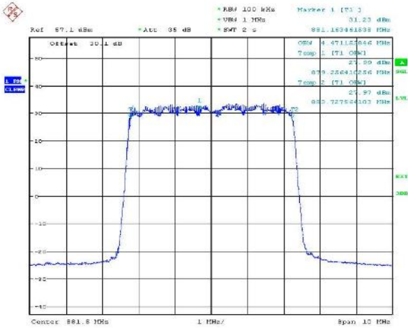
Figure 93 Occupied Bandwidth – QPSK (881.5 MHz) (5MHz Channel BW)
