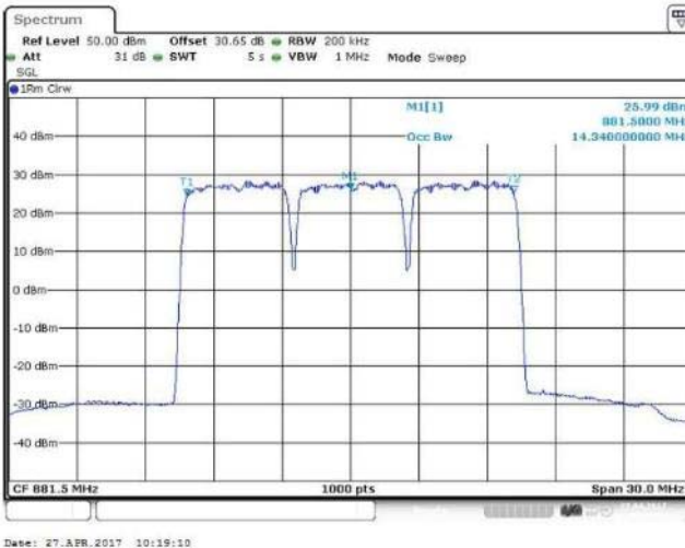
Figure 54 Occupied Bandwidth – 16QAM (876.5, 881.5, 886.5 MHz)) (3 X 5 MHz Channel BW)
