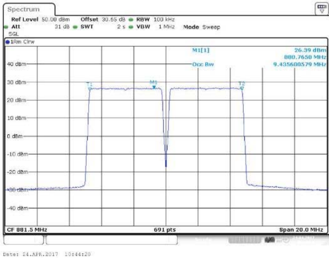
Figure 35 Occupied Bandwidth – 64QAM (879 MHz, 884 MHz) (2 X 5 MHz Channel BW)
