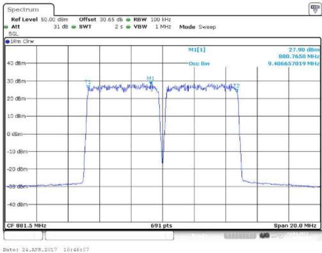
Figure 34 Occupied Bandwidth – 16QAM (879 MHz, 884 MHz) (2 X 5 MHz Channel BW)
