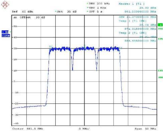
Figure 109 Occupied Bandwidth – QPSK (876.5/881.5/886.5 MHz) (5+5+5MHz Channel BW)
