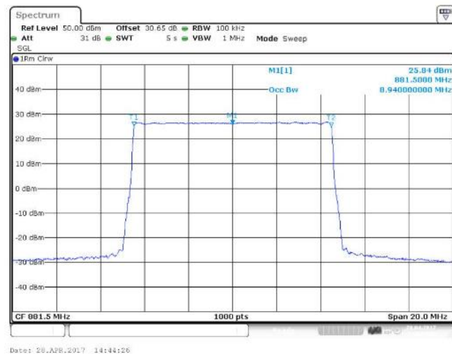
Figure 68 Occupied Bandwidth – 256QAM (881.5 MHz) (1 X 10 MHz Channel BW)
