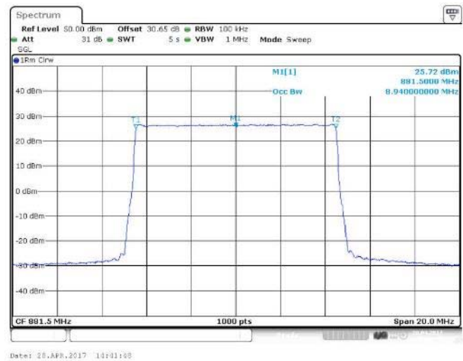
Figure 67 Occupied Bandwidth – 64QAM (881.5 MHz) (1 X 10 MHz Channel BW)
