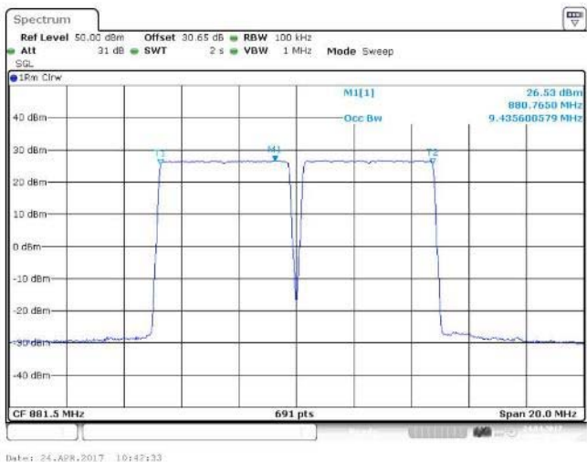
Figure 33 Occupied Bandwidth – QPSK (879 MHz, 884 MHz) (2 X 5 MHz Channel BW)
