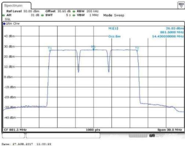
Figure 52 Occupied Bandwidth – 256QAM (881.5 MHz) (3 X 5 MHz Channel BW)
