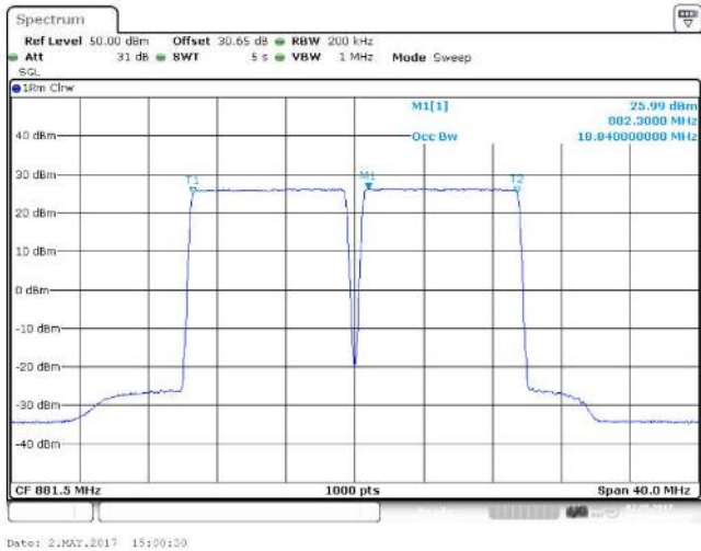
Figure 80 Occupied Bandwidth – 256QAM (876.5 MHz, 886.5 MHz) (2 X 10 MHz Channel BW)
