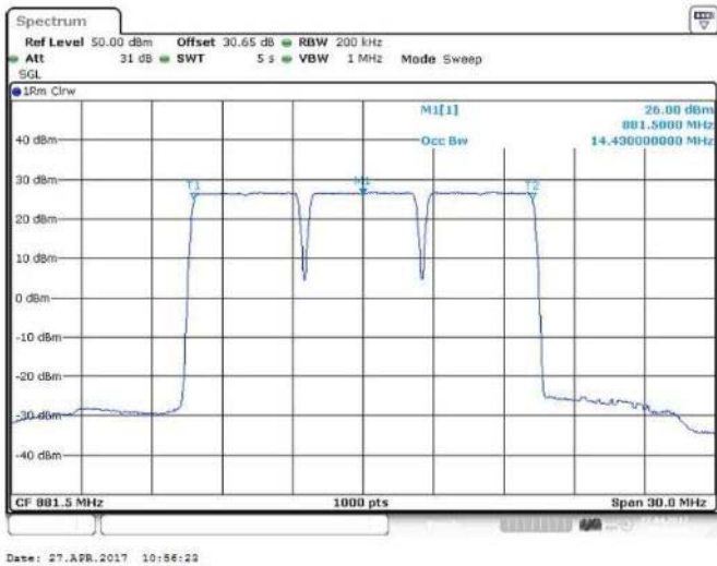
Figure 48 Occupied Bandwidth – 256QAM (876.5, 881.5, 886.5 MHz) (3 X 5 MHz Channel BW)
