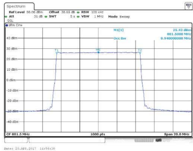
Figure 75 Occupied Bandwidth – 64QAM (881.5 MHz) (1 X 10 MHz Channel BW)
