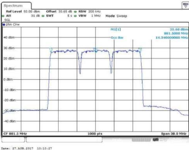
Figure 50 Occupied Bandwidth – 16QAM (876.5, 881.5, 886.5 MHz) (3 X 5 MHz Channel BW)
