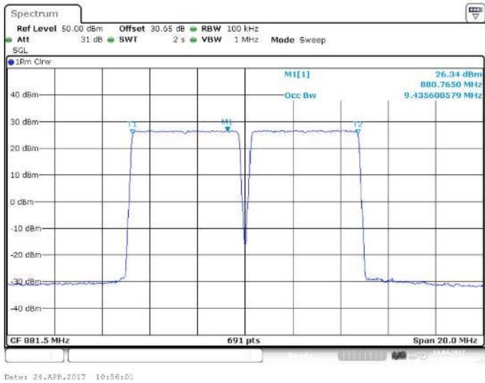
Figure 39 Occupied Bandwidth – 64QAM (879 MHz, 884 MHz) (2 X 5 MHz Channel BW)
