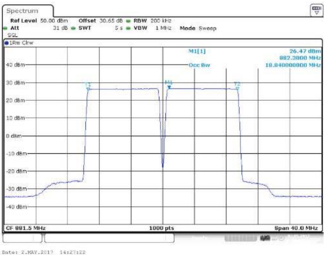
Figure 81 Occupied Bandwidth – QPSK (876.5 MHz, 886.5 MHz) (2 X 10 MHz Channel BW)
