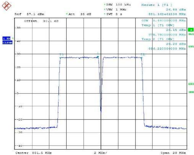
Figure 107 Occupied Bandwidth – 64QAM (879/884 MHz) (5+5MHz Channel BW)
