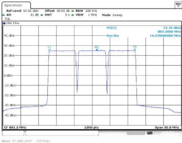
Figure 51 Occupied Bandwidth – 64QAM ((876.5, 881.5, 886.5 MHz)) (3 X 5 MHz Channel BW)
