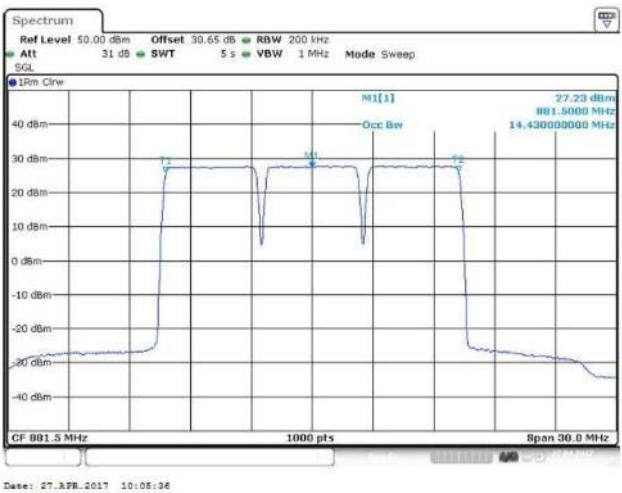
Figure 49 Occupied Bandwidth – QPSK (876.5, 881.5, 886.5 MHz) (3 X 5 MHz Channel BW)
