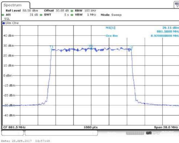
Figure 74 Occupied Bandwidth – 16QAM (881.5 MHz) (1 X 10 MHz Channel BW)
