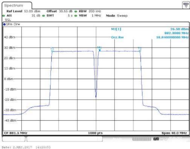
Figure 83 Occupied Bandwidth – 64QAM (876.5 MHz, 886.5 MHz) (2 X 10 MHz Channel BW)
