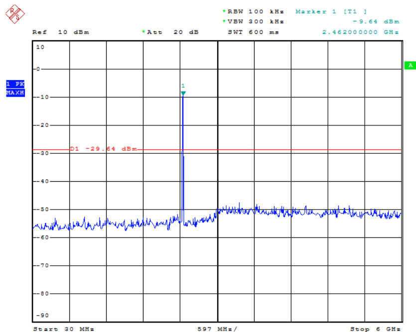
Figure 23: Conducted Spurious Emission, 30MHz –6GHz, Mode C
