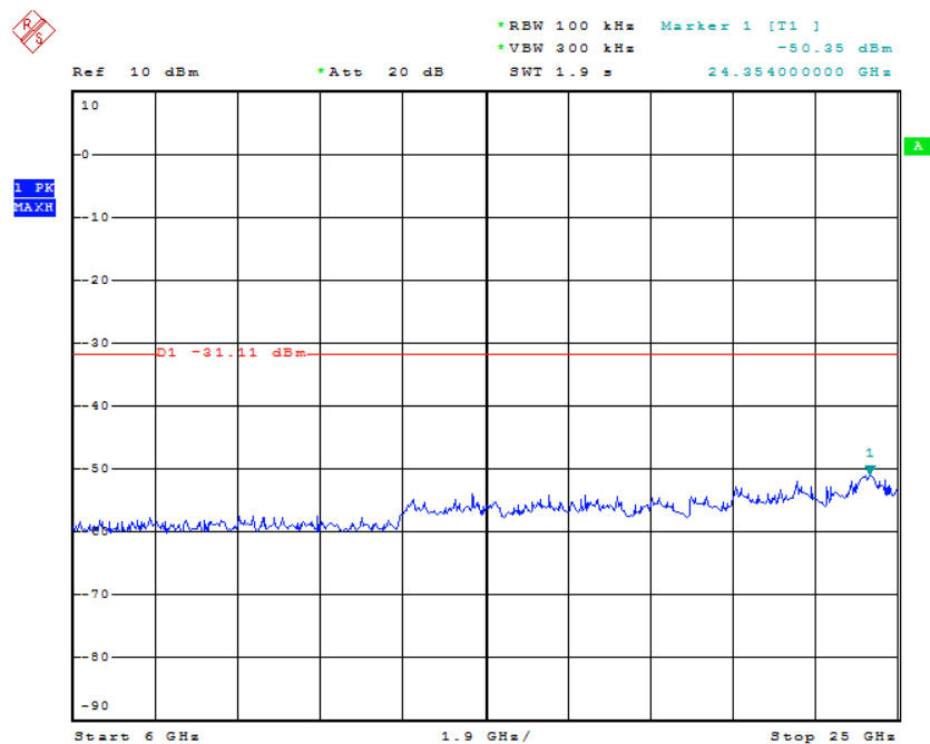
Figure 20: Conducted Spurious Emission, 6GHz – 25GHz, Mode A
