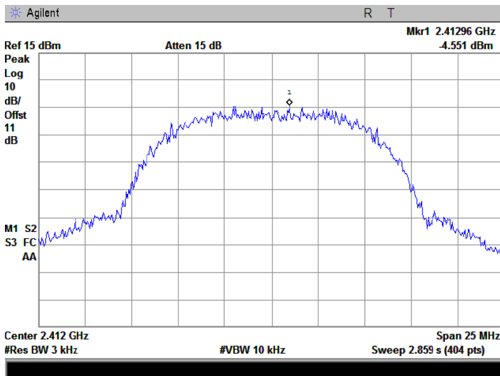
Figure 25: Power spectral density, 802.11 B, Mode A
