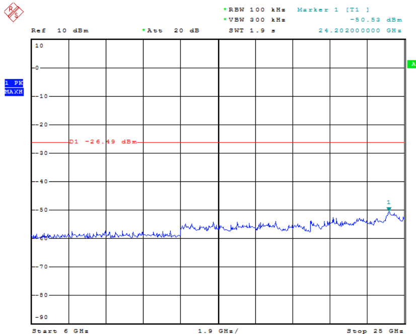
Figure 18: Conducted Spurious Emission, 6GHz – 25GHz, Mode C
