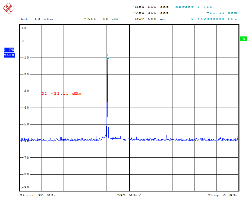
Figure 19: Conducted Spurious Emission, 30MHz – 6GHz, Mode A
