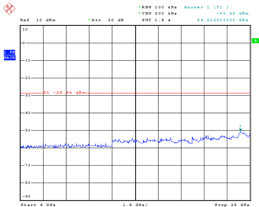
Figure 24: Conducted Spurious Emission, 6GHz – 25GHz, Mode C
