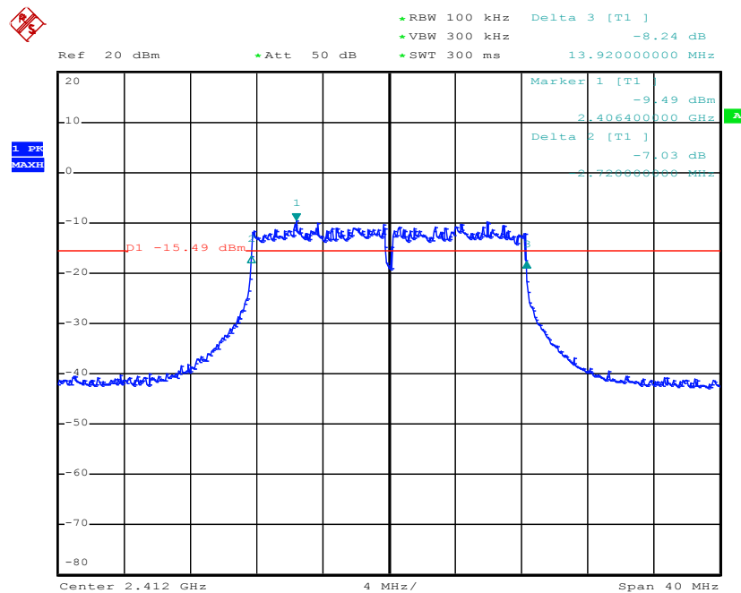
Figure 10: 6 dB Bandwidth of 802.11G, Mode A
