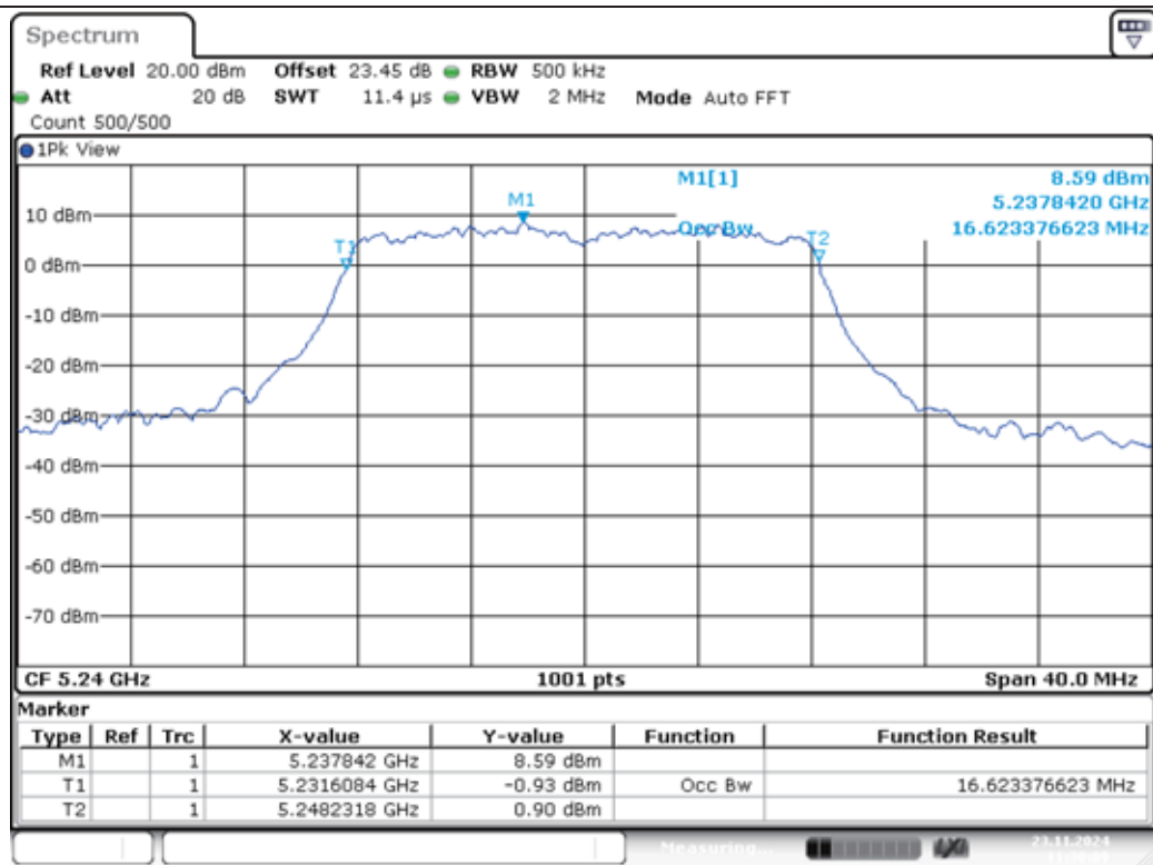
11A-Ant1-5240
