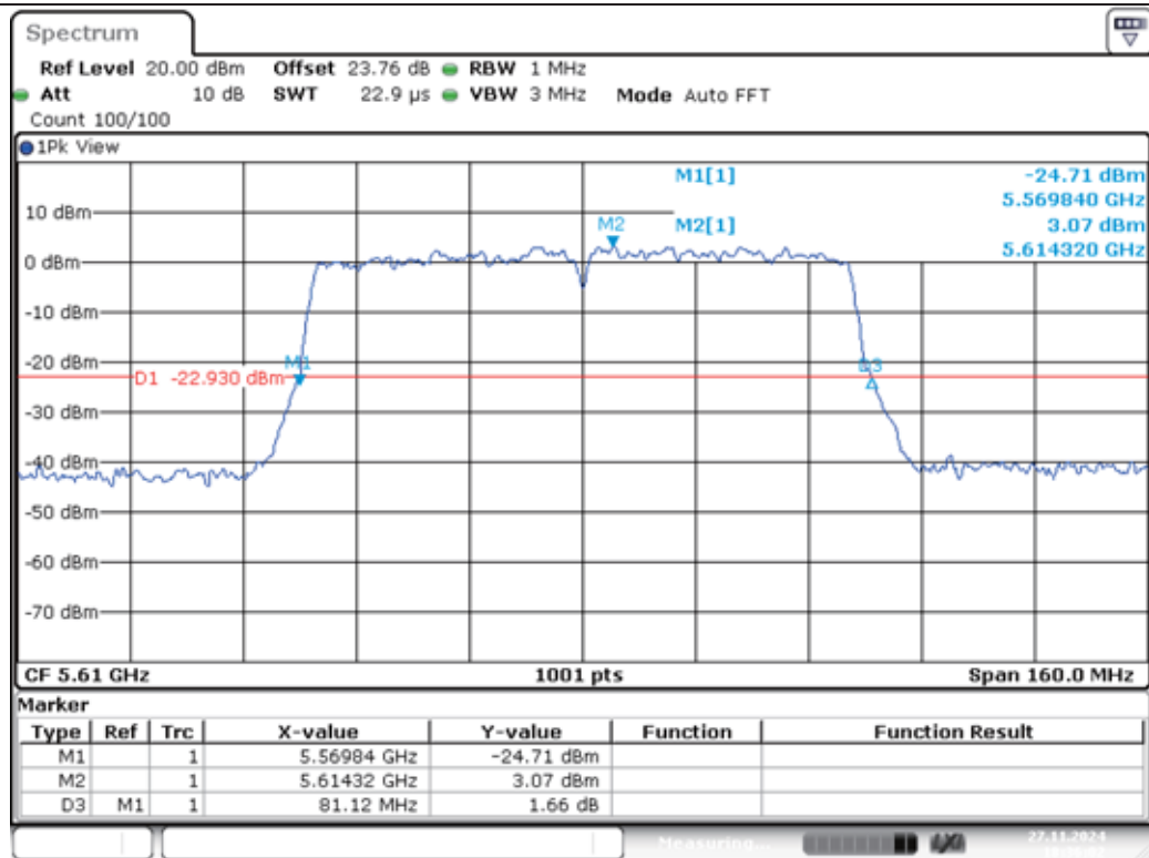
11AC80MIMO-Ant1-5610
