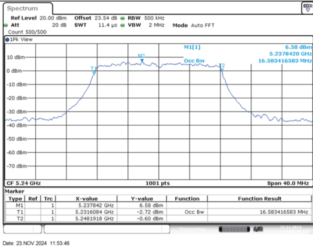
11A-Ant2-5240
