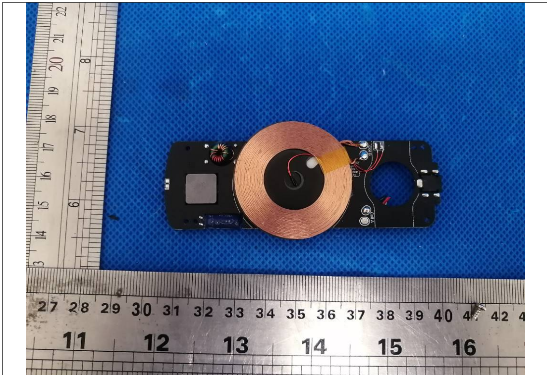
Figure 3. PCB view
