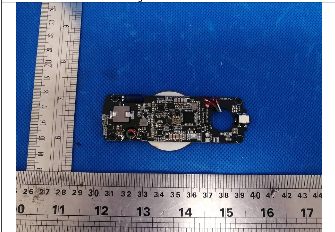
Figure 2. PCB view
