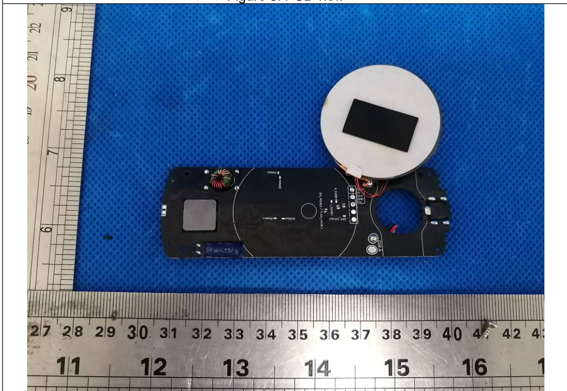
Figure 4. PCB view
