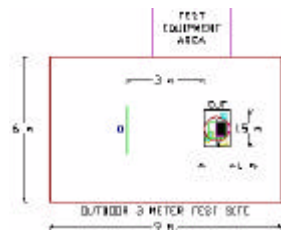
Figure 7. Dimensions of Outdoor Test Site
