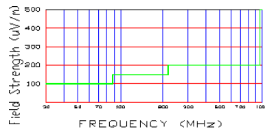
Figure 10. Limits at 3 meters
