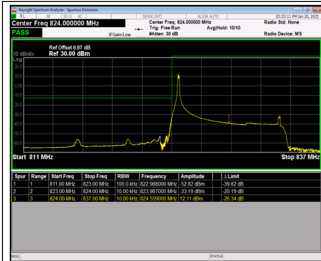
Band5-10MHz-QPSK-20450-50RB#0
