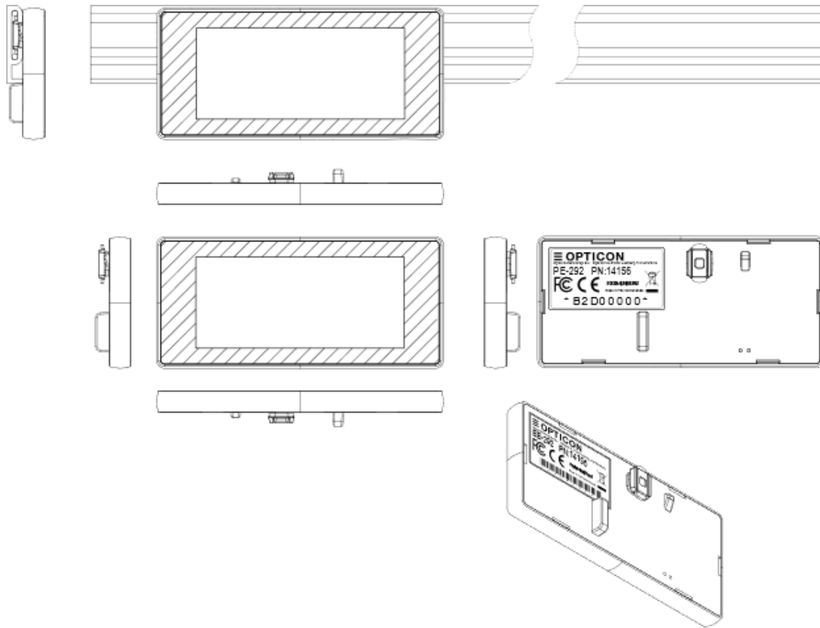
Figure 8: Mechanical drawing
