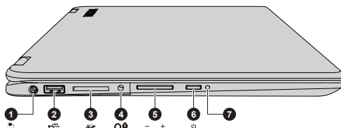
Figure 3-2 The left side of the computer
