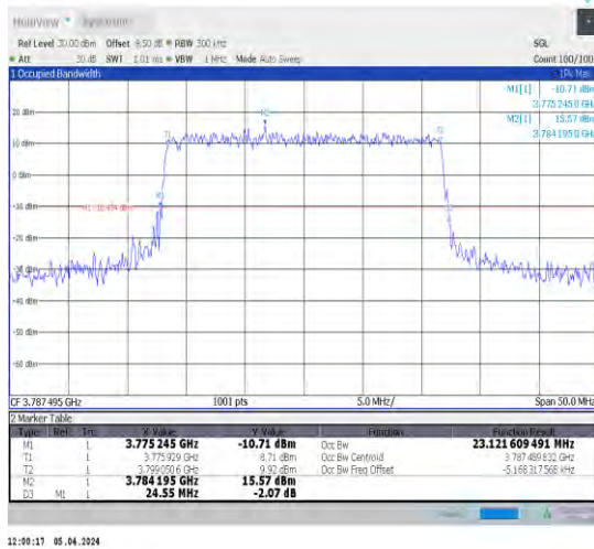
1-N78-3700-3800-N78-3700-380030-25-H-6-CP-QP SK-Outer_Full-65@0-Ant1-23.122-24.550-≤25-PASS
