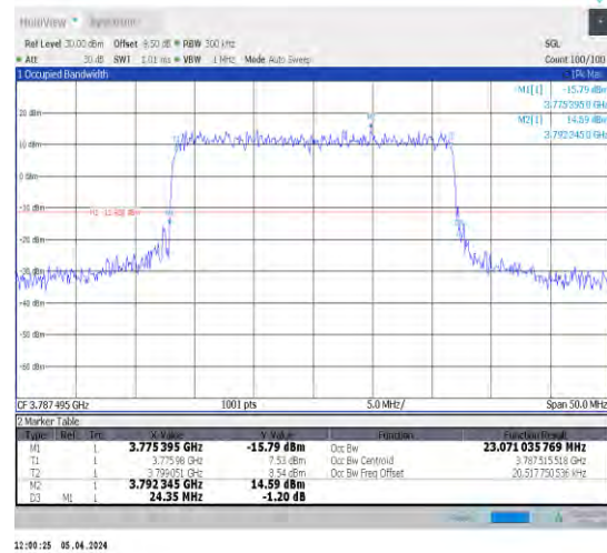
1-N78-3700-3800-N78-3700-380030-25-H-7-CP-16 QAM-Outer_Full-65@0-Ant1-23.071-24.350-≤25-PA SS
