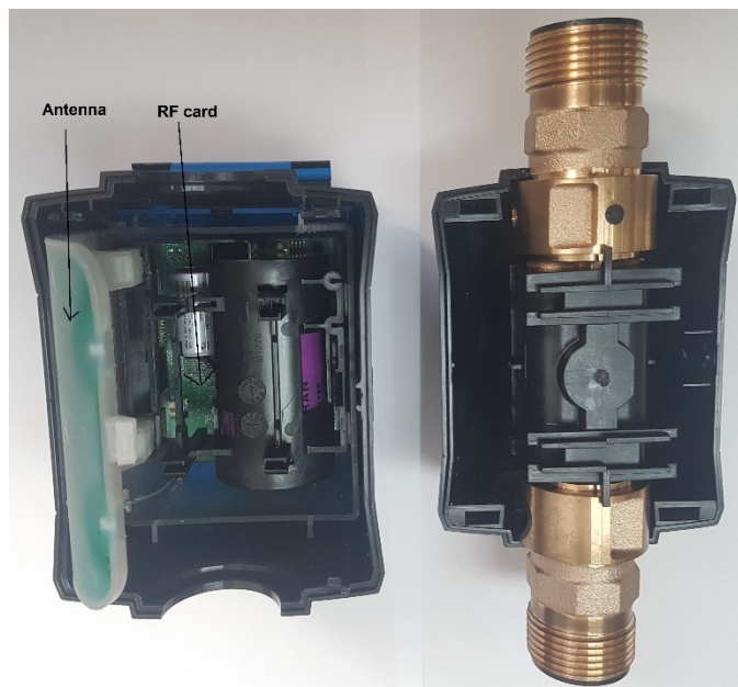
Assembly
