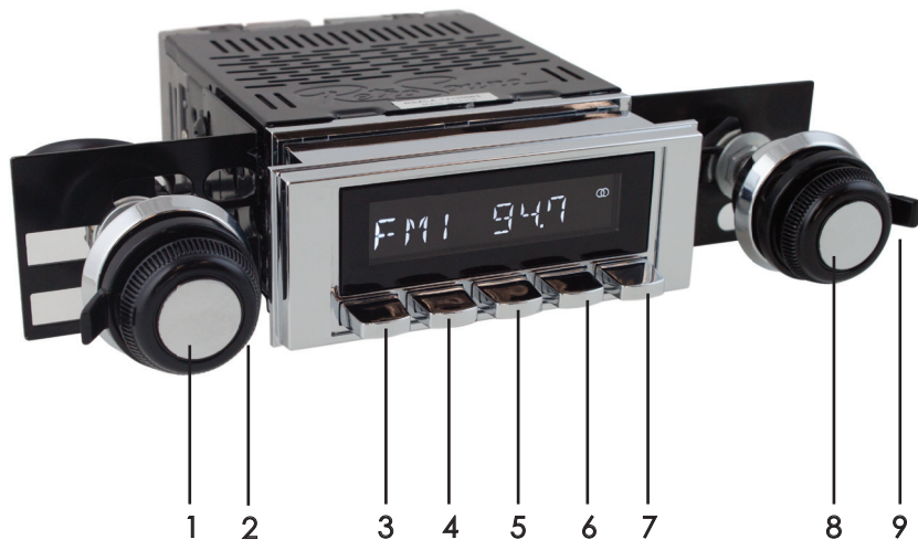
Figure 7 - Radio Controls
