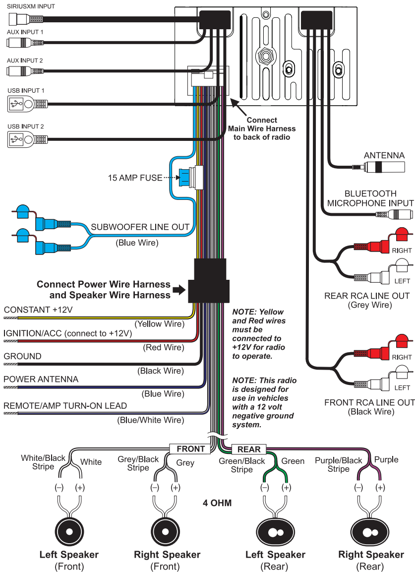
Figure 5 - Wiring Diagram
