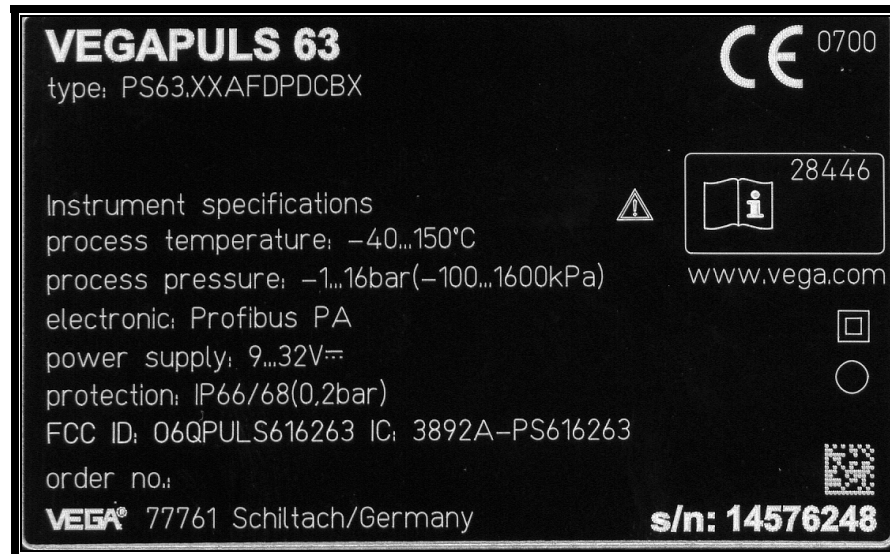
Photograph 3: FCC ID/IC ID Label Sample for Model VEGAPULS 63
