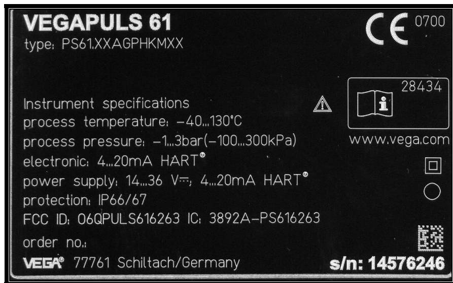
Photograph 1: FCC ID/IC ID Label Sample for Model VEGAPULS 61
