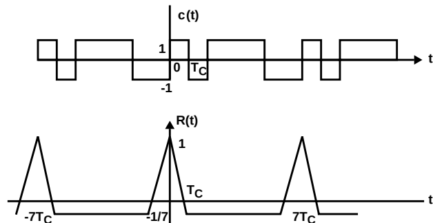
FIGURE 20. SEVEN CHIP M-SEQUENCE AND ITS AUTOCORRELATION FUNCTION
