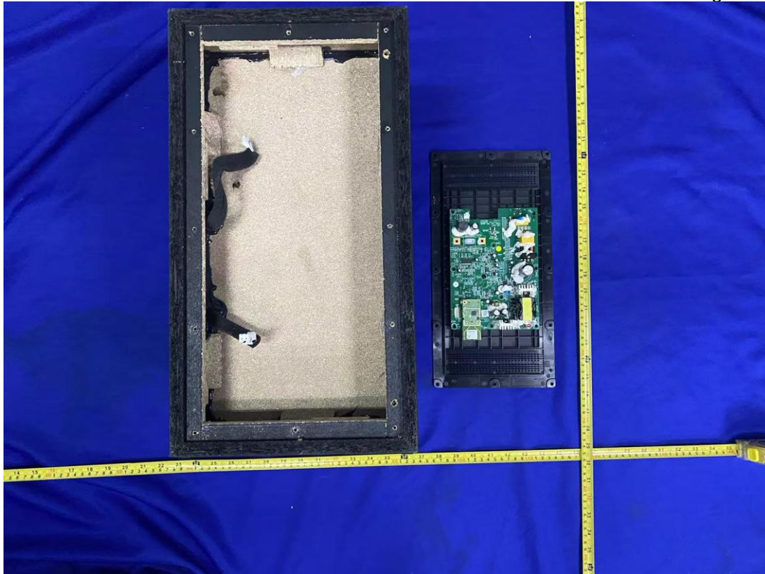
Figure 1 Inside Configuration of the EUT
