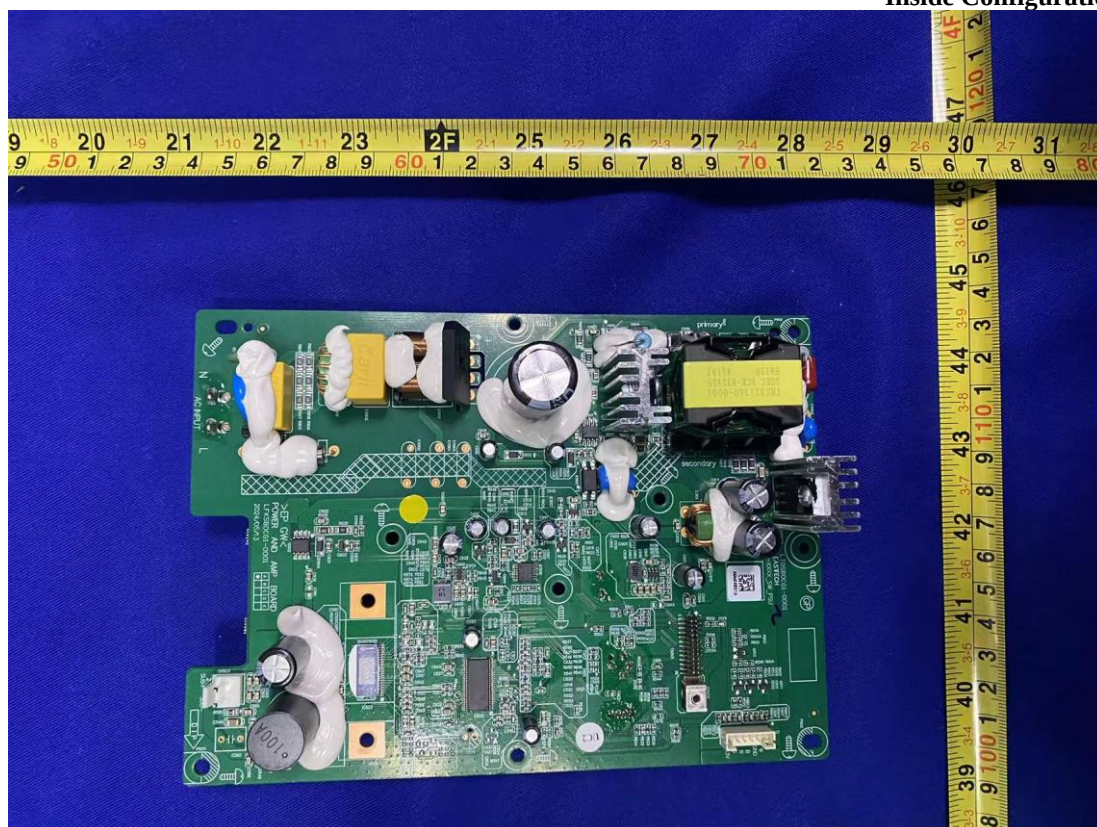
Figure 3 Inside Configuration of the EUT
