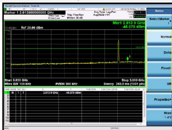
802.11n-20 CHANNEL 1, SPURIOUS 30 MHz ~ 3 GHz
