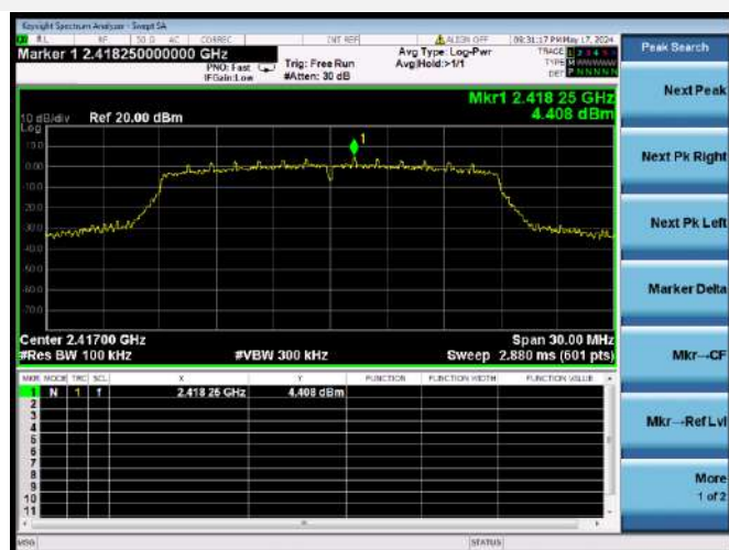
802.11n-20 CHANNEL 2 CARRIER LEVEL
