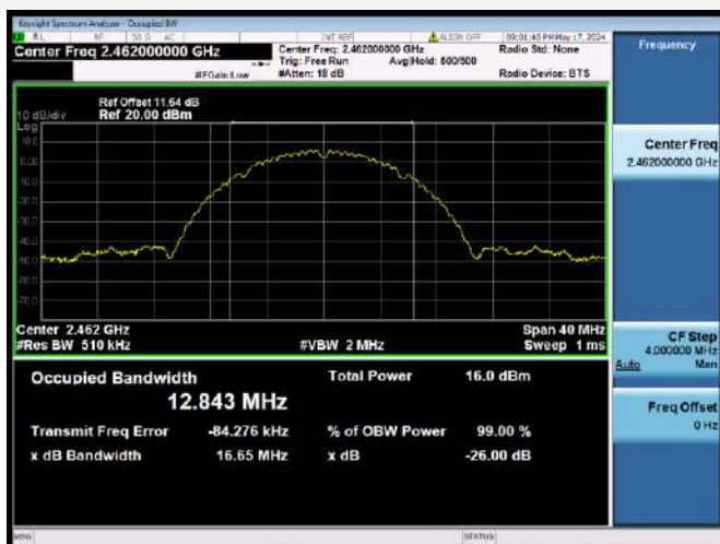
802.11b CHANNEL 11
