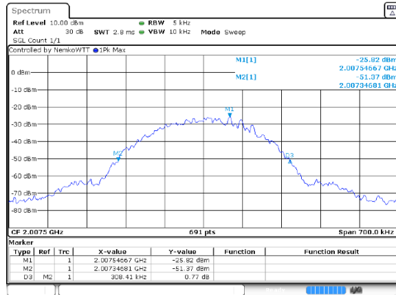
Figure 8.3-5: Occupied bandwidth / Input Versus Output Comparison results, narrowband signal, 0.5 dB below AGC threshold, input and output signal respectively
