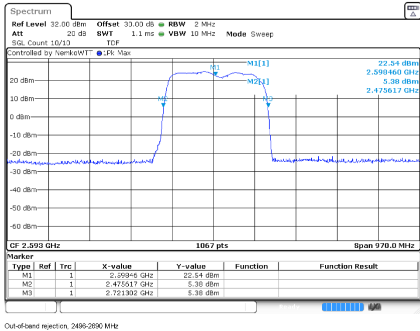
Figure 8.2-4: Out of band rejection results, Band 41
