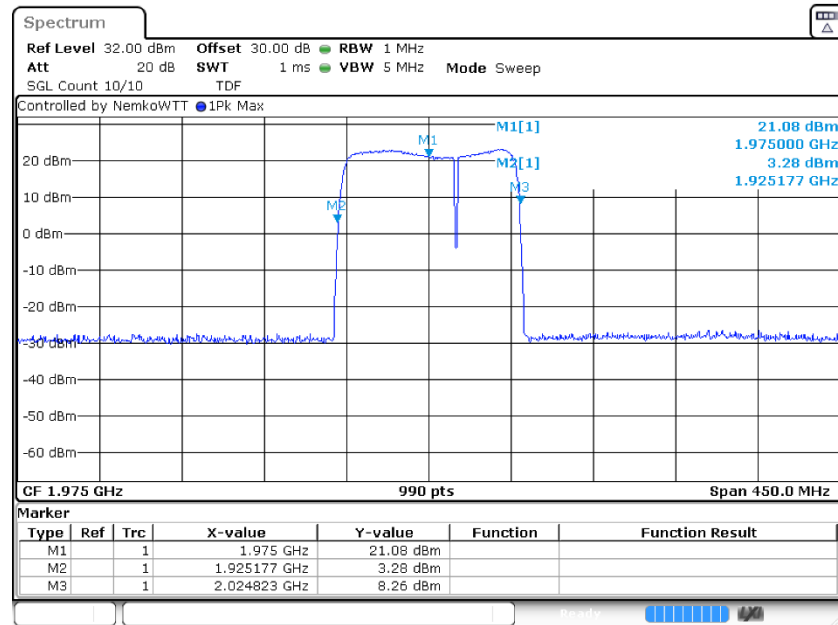
Figure 8.2-1: Out of band rejection results, Band 25_Band 70
