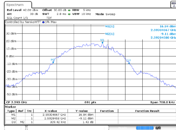
Figure 8.3-17: Occupied bandwidth / Input Versus Output Comparison results, narrowband signal, 0.5 dB below AGC threshold, input and output signal respectively
