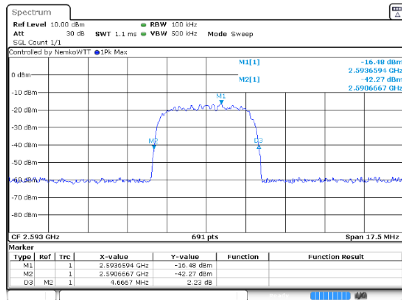
Figure 8.3-19: Occupied bandwidth / Input Versus Output Comparison results, broadband signal, 0.5 dB below AGC threshold, input and output signal respectively
