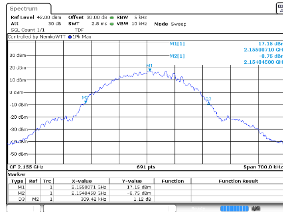
Figure 8.3-9: Occupied bandwidth / Input Versus Output Comparison results, narrowband signal, 0.5 dB below AGC threshold, input and output signal respectively
