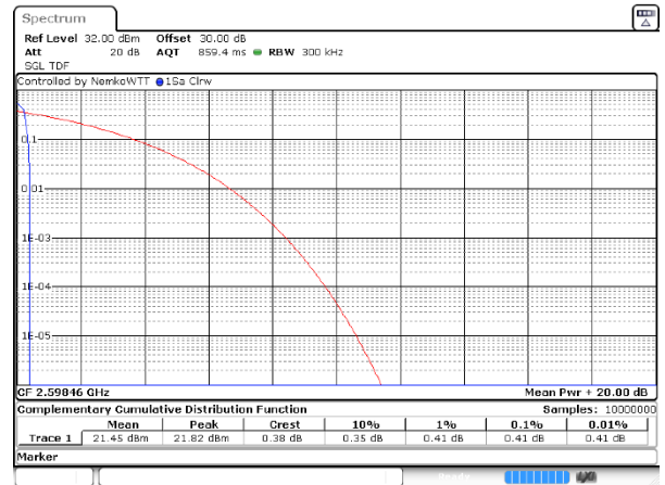
Figure 8.4-17: Output power / Mean output power and amplifier gain results, narrowband signal, 0.5 dB below AGC threshold, input and output signal respectively
