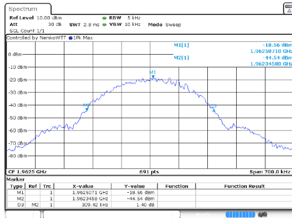
Figure 8.3-1: Occupied bandwidth / Input Versus Output Comparison results, narrowband signal, 0.5 dB below AGC threshold, input and output signal respectively
