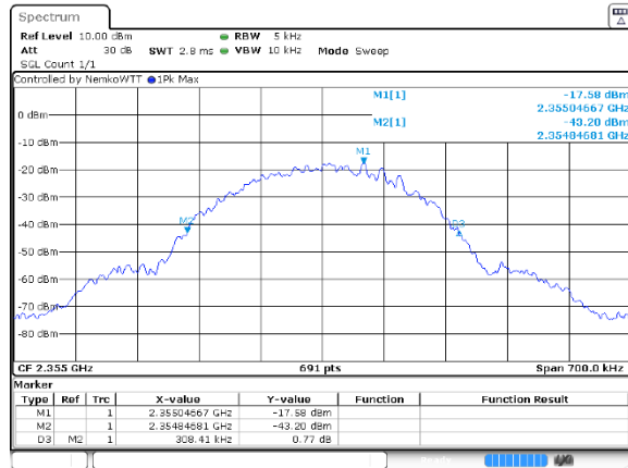
Figure 8.3-13: Occupied bandwidth / Input Versus Output Comparison results, narrowband signal, 0.5 dB below AGC threshold, input and output signal respectively
