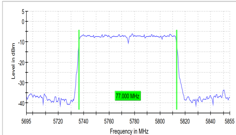
99 % Bandwidth
