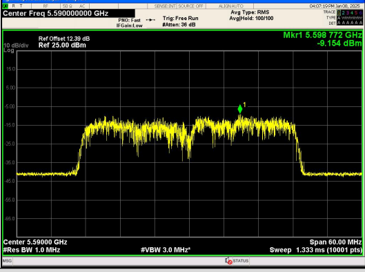
IEEE 802.11n Channel 118 40MHz Antenna 0
