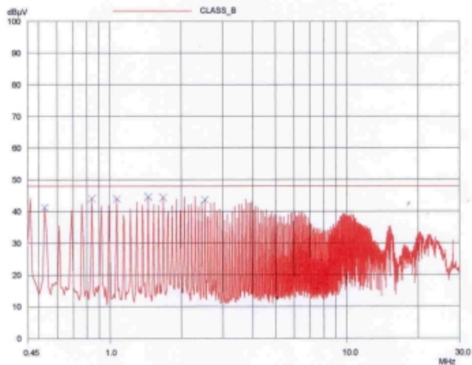
HOT LINE
