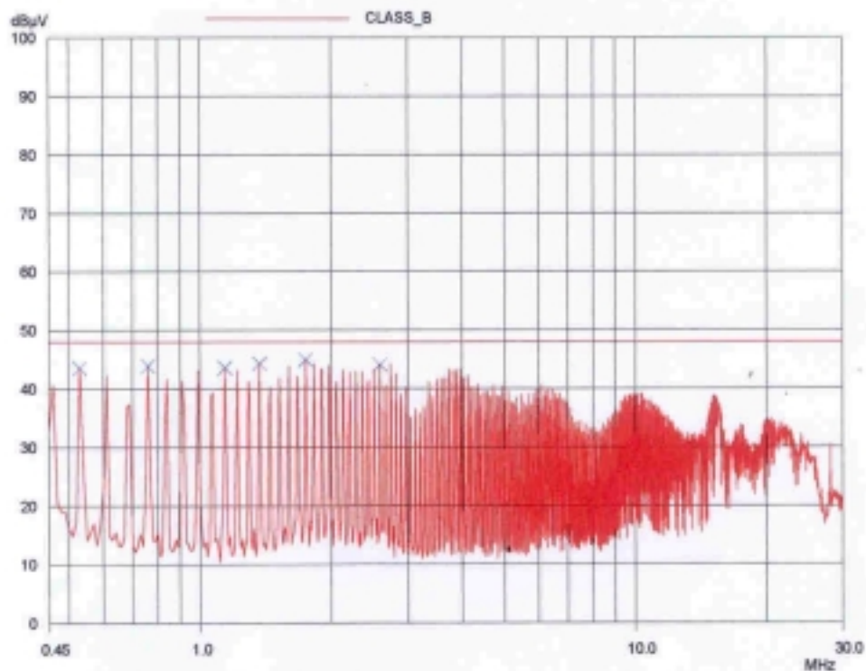
NEUTRAL LINE
