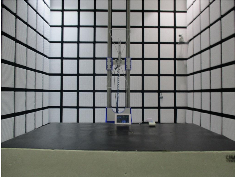
Radiated Emission
