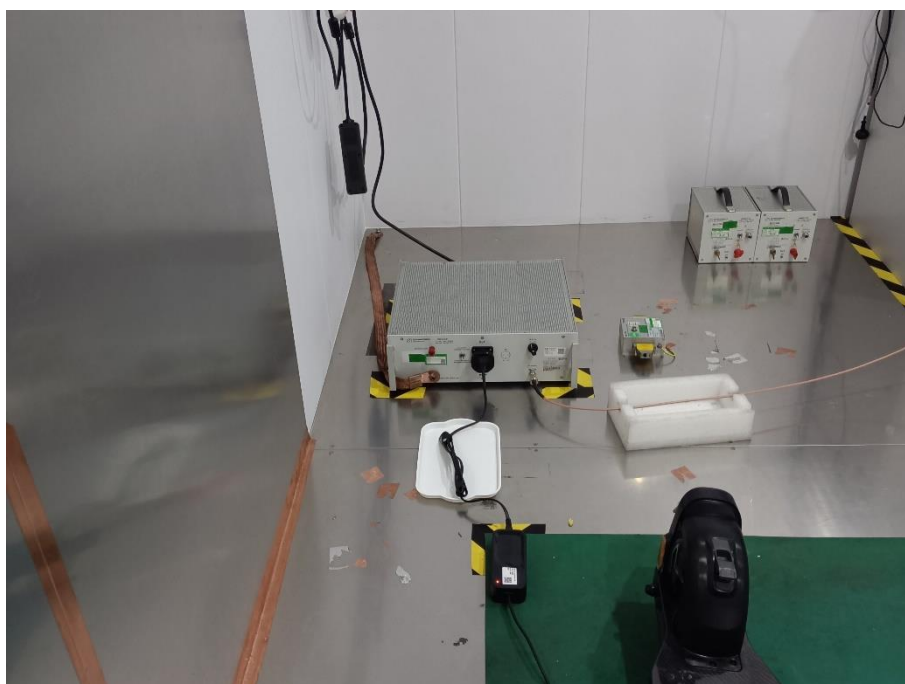
Conducted Emission-1
