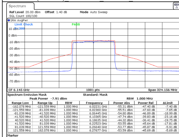
802.11ax (80MHz) 6145MHz Chain A NSS-2
