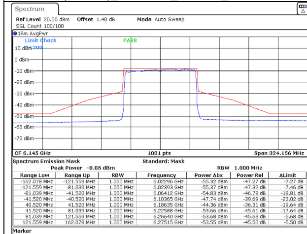
802.11ax (80MHz) 6145MHz Chain C NSS-2
