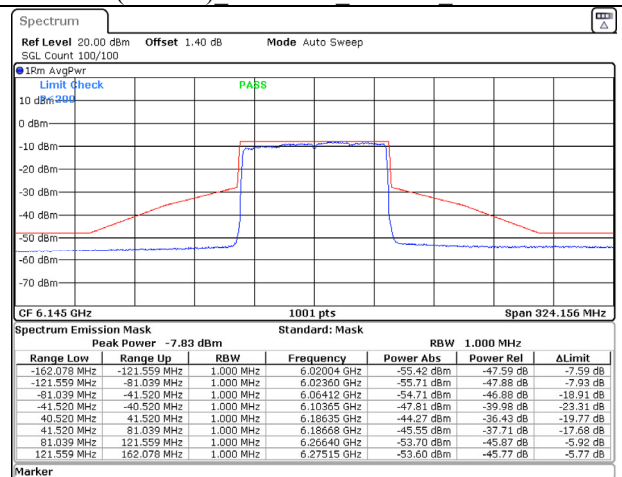
802.11ax (80MHz) 6145MHz Chain B NSS-2
