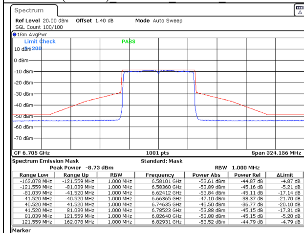
802.11ax (80MHz) 6705MHz Chain A NSS-2
