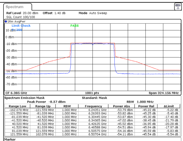
802.11ax (80MHz) 6385MHz Chain D NSS-2
