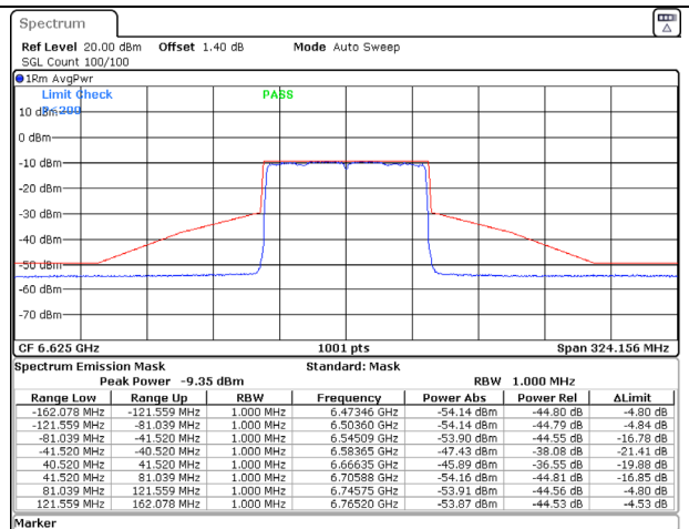
802.11ax (80MHz) 6625MHz Chain D NSS-2
