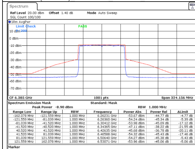
802.11ax (80MHz) 6385MHz Chain A NSS-2
