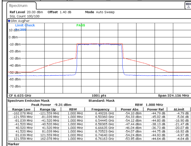
802.11ax (80MHz) 6625MHz Chain A NSS-2
