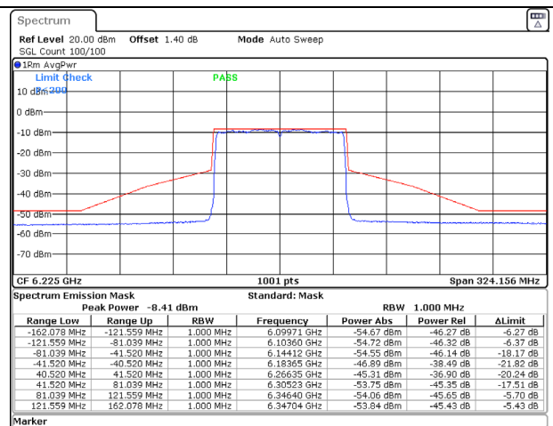
802.11ax (80MHz) 6225MHz Chain B NSS-2
