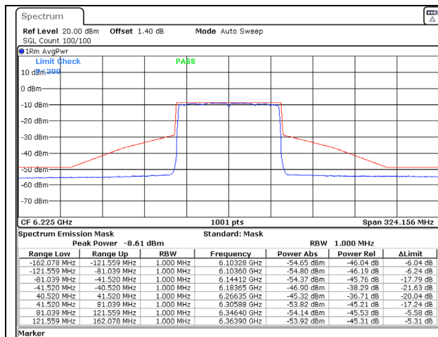
802.11ax (80MHz) 6225MHz Chain A NSS-2
