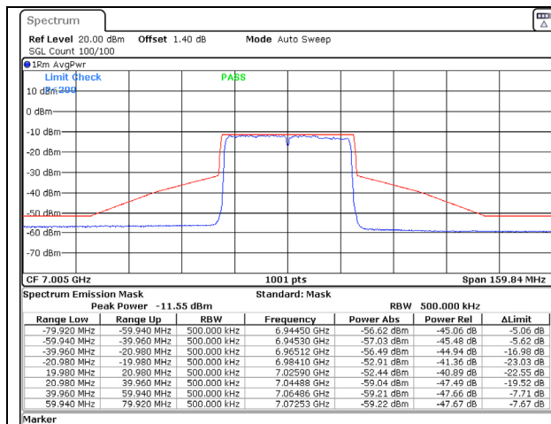
802.11ax (40MHz) 7005MHz Chain A NSS-2
