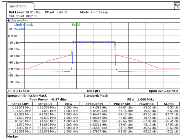
802.11ax (80MHz) 6545MHz Chain A NSS-2
