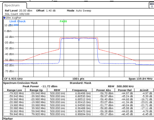
802.11ax (40MHz) 6925MHz Chain A NSS-2
