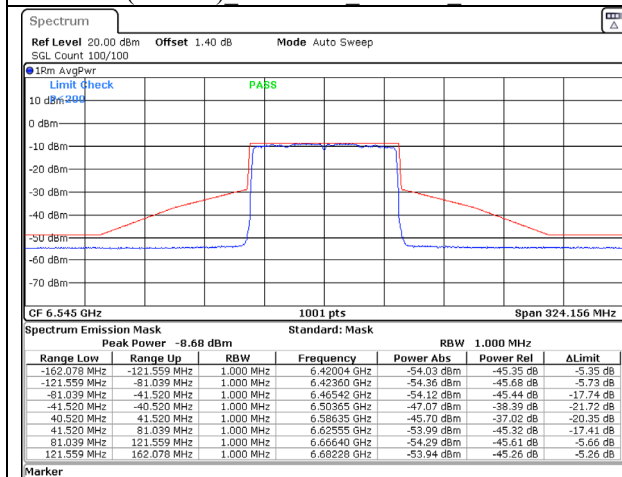
802.11ax (80MHz) 6545MHz Chain C NSS-2
