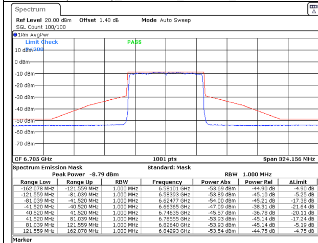
802.11ax (80MHz) 6705MHz Chain C NSS-2
