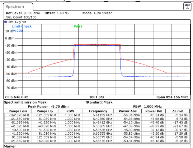
802.11ax (80MHz) 6545MHz Chain D NSS-2
