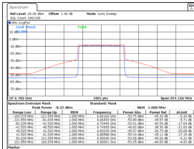
802.11ax (80MHz) 6785MHz Chain A NSS-2
