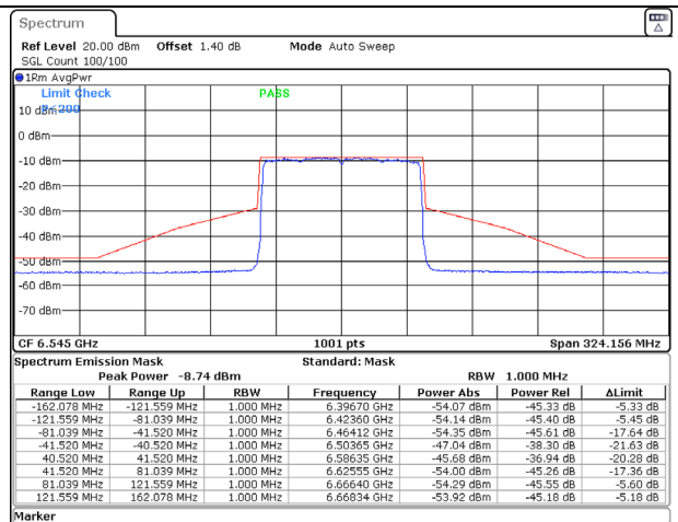
802.11ax (80MHz) 6545MHz Chain B NSS-2
