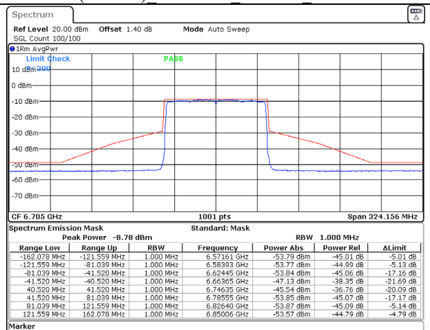
802.11ax (80MHz) 6705MHz Chain B NSS-2
