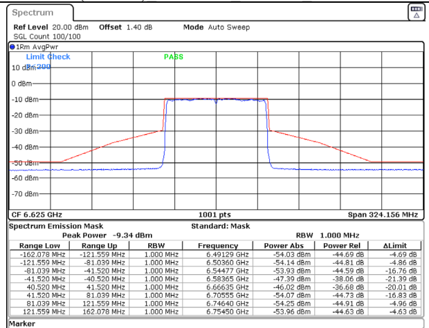
802.11ax (80MHz) 6625MHz Chain B NSS-2
