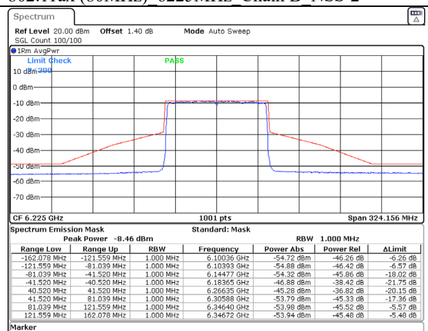
802.11ax (80MHz) 6225MHz Chain D NSS-2
