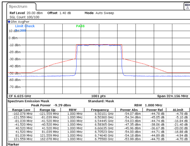
802.11ax (80MHz) 6625MHz Chain C NSS-2
