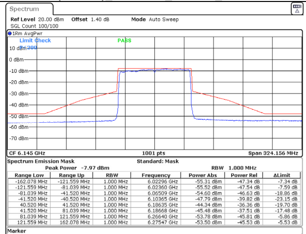
802.11ax (80MHz) 6145MHz Chain D NSS-2
