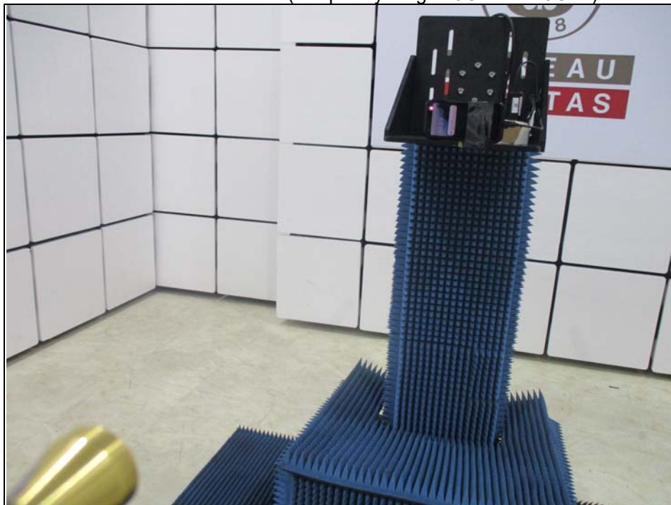
Radiated Emission Test (Frequency range 75GHz ~ 110GHz)
