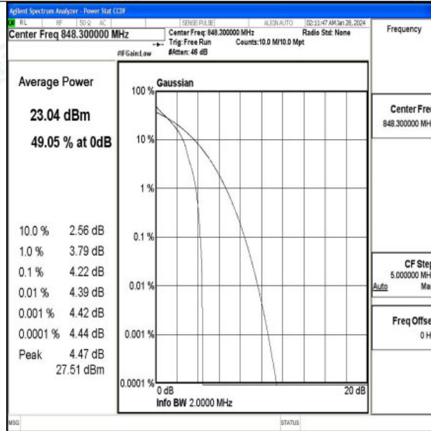
Band5-1.4MHz-QPSK-20643-1RB#0-PASS
