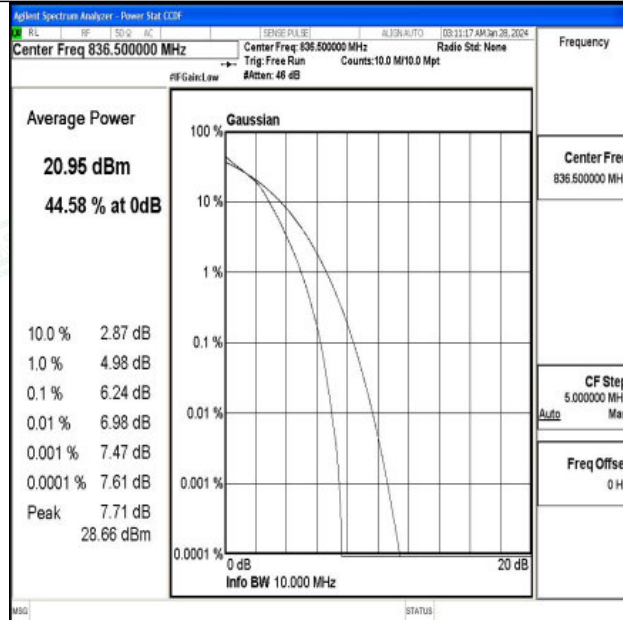
Band5-10MHz-16QAM-20525-50RB#0-PASS
