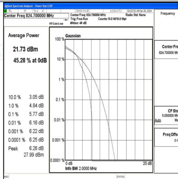
Band5-1.4MHz-16QAM-20407-1RB#0-PASS
