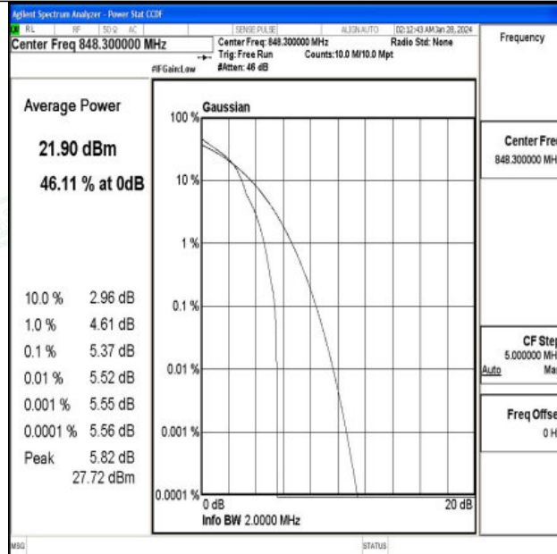
Band5-1.4MHz-16QAM-20643-1RB#0-PASS
