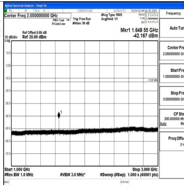
Band5_1.4MHz_16QAM_20407_1RB#0_1000~3000_1000~3000
