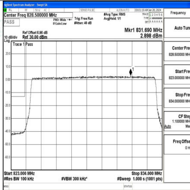
Band5_10MHz_16QAM_20450_50RB#0
