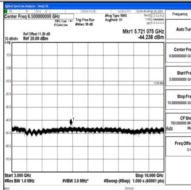
Band5_1.4MHz_16QAM_20407_1RB#0_3000~10000_3000~10000
