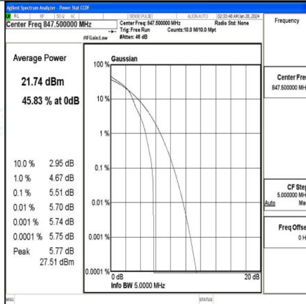
Band5-3MHz-16QAM-20635-1RB#0-PASS
