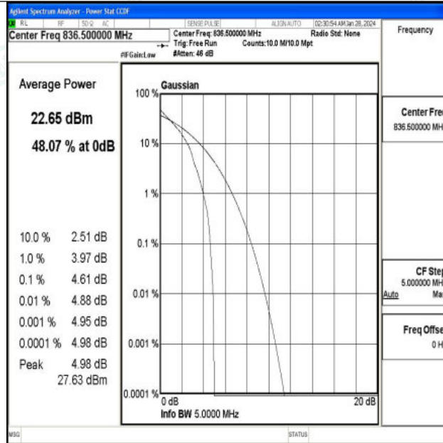
Band5-3MHz-QPSK-20525-1RB#0-PASS
