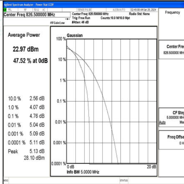
Band5-5MHz-QPSK-20425-1RB#0-PASS
