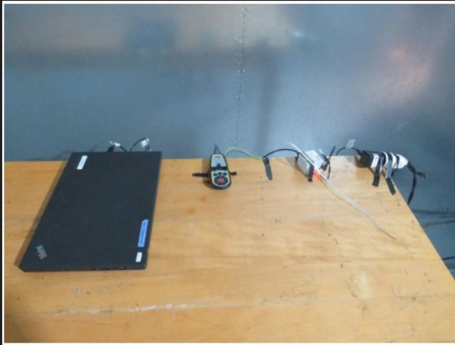
Setup for measurements 150 kHz - 30 MHz
