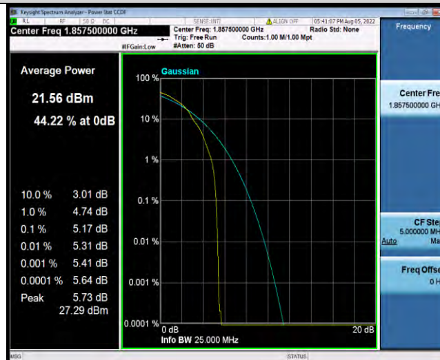
Band2-15MHz-64QAM-18675-75RB#0
