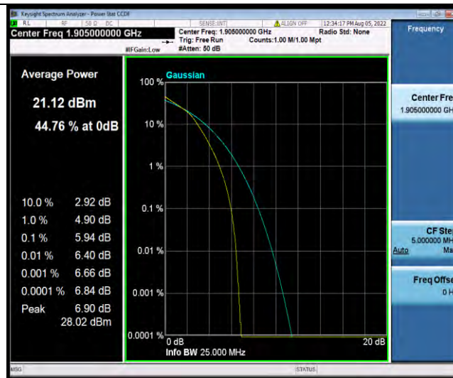
Band2-10MHz-64QAM-18650-1RB#0
