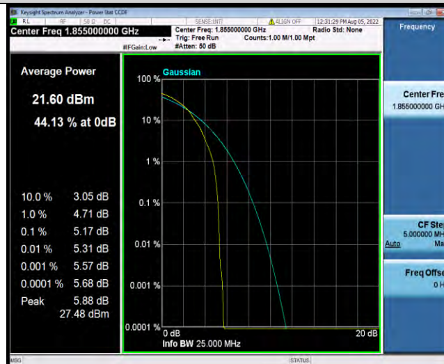
Band2-10MHz-64QAM-18650-50RB#0
