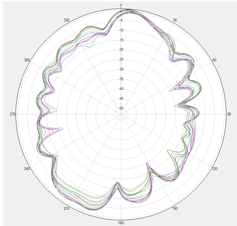
5G WIFI \Phi=90\text{deg}
