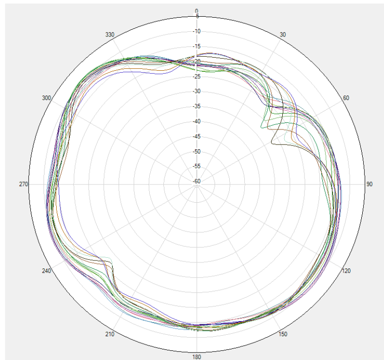
5G WIFI \Theta=90\text{deg}
