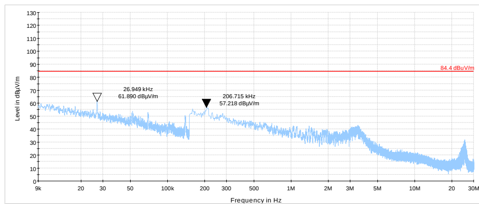
Plot 7.5.2 Radiated emission measurements in 0.009-30 MHz range
