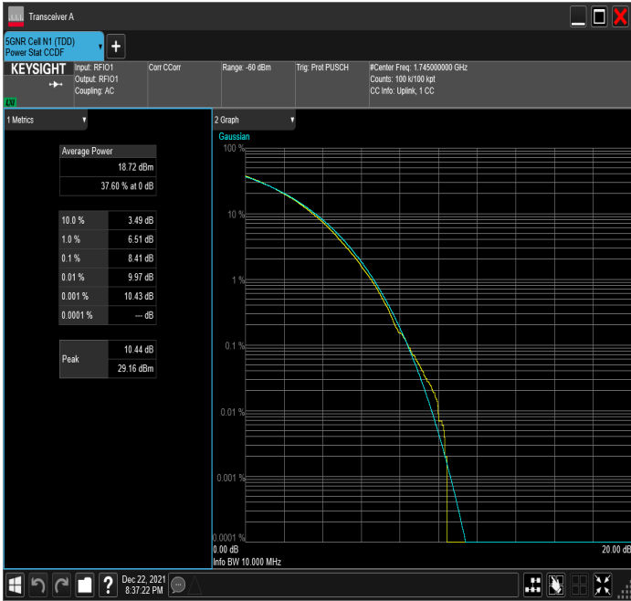
n66_10MHz_15kHz_1745MHz_CP-OFDM 256 QAM_RB52@0
