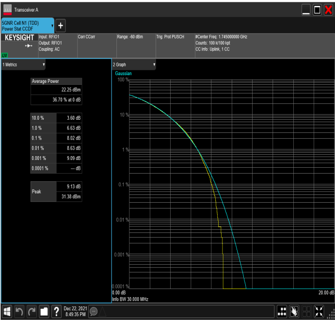
n66_30MHz_15kHz_1745MHz_CP-OFDM QPSK_RB160@0
