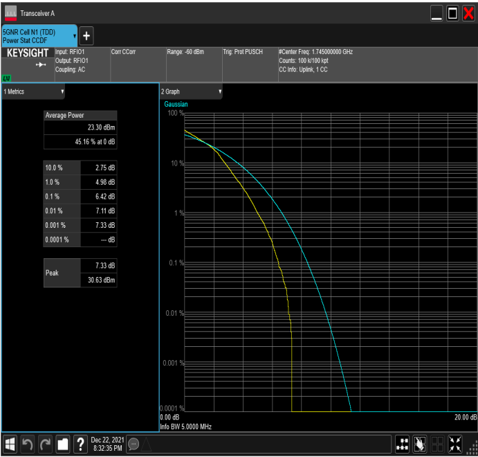
n66_5MHz_15kHz_1745MHz_DFT-s-OFDM 16 QAM_RB25@0
