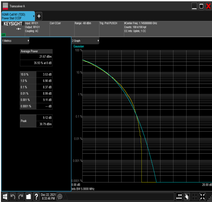
n66_5MHz_15kHz_1745MHz_CP-OFDM 64 QAM_RB25@0
