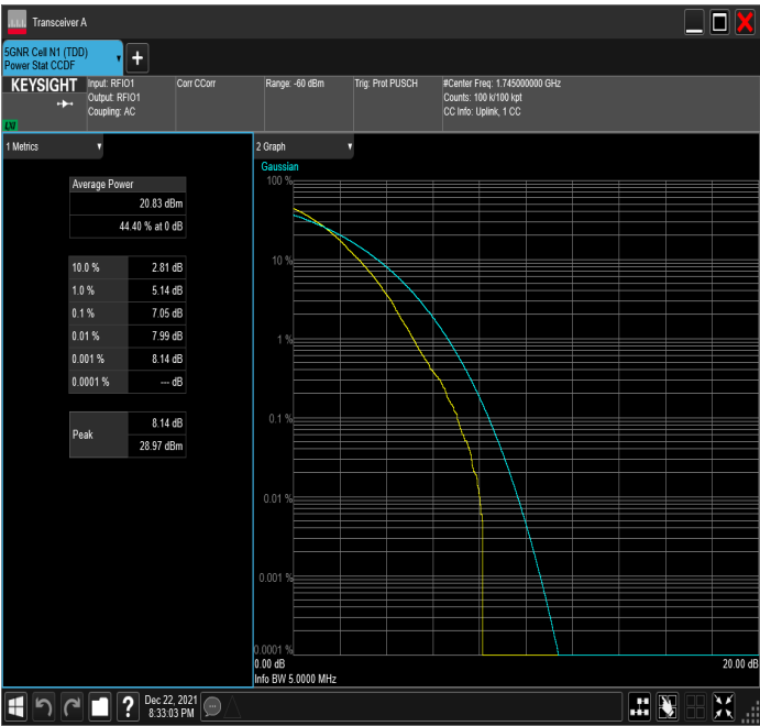
n66_5MHz_15kHz_1745MHz_DFT-s-OFDM 256 QAM_RB25@0
