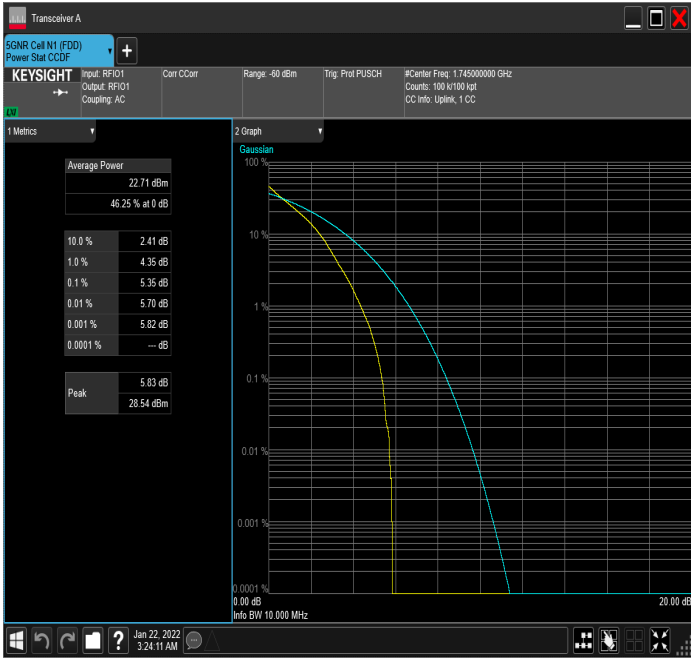
n66_10MHz_15kHz_1745MHz_CP-OFDM QPSK_RB52@0
