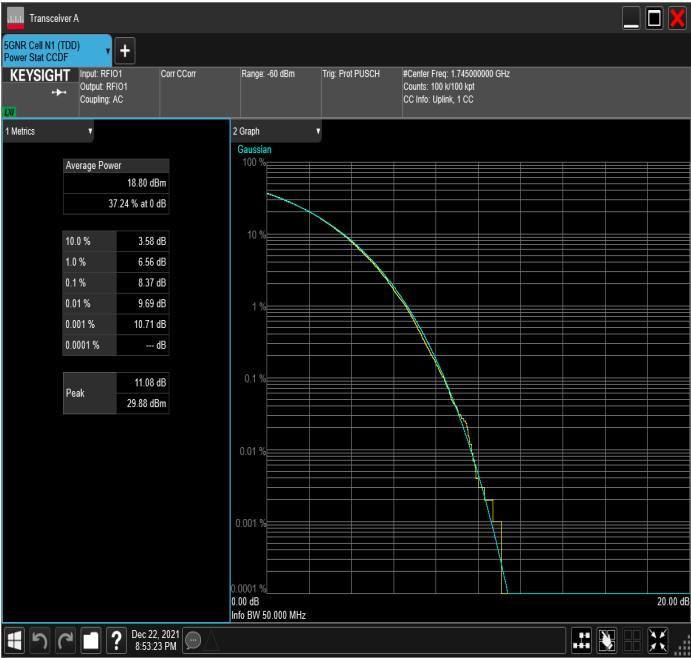
n66_40MHz_15kHz_1745MHz_CP-OFDM 256 QAM_RB216@0
