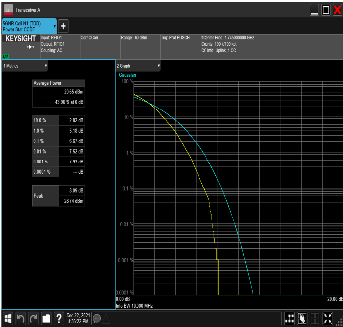
n66_10MHz_15kHz_1745MHz_DFT-s-OFDM 256 QAM_RB50@0
