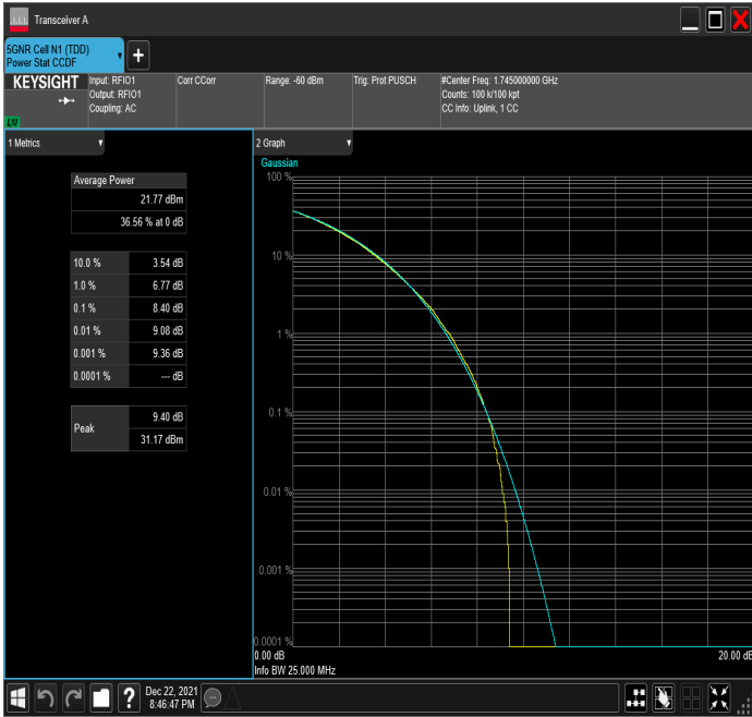
n66_25MHz_15kHz_1745MHz_CP-OFDM 64 QAM_RB133@0
