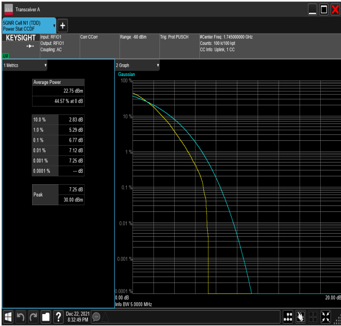
n66_5MHz_15kHz_1745MHz_DFT-s-OFDM 64 QAM_RB25@0
