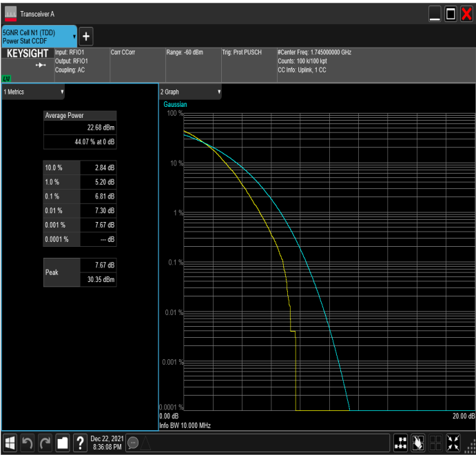
n66_10MHz_15kHz_1745MHz_DFT-s-OFDM 64 QAM_RB50@0
