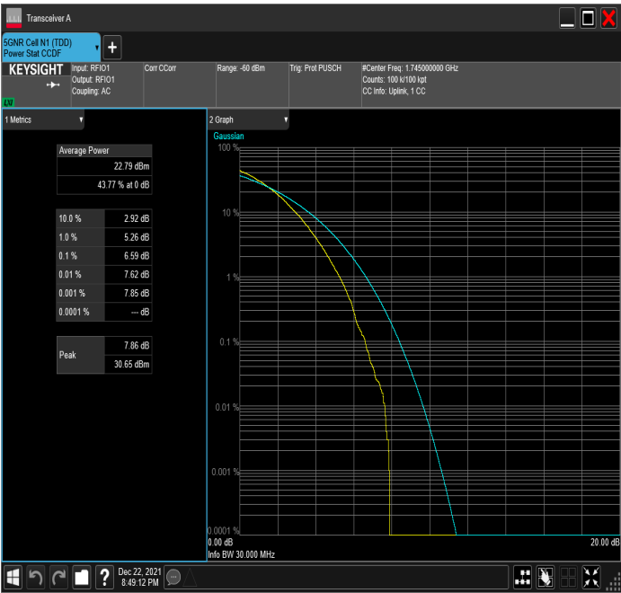
n66_30MHz_15kHz_1745MHz_DFT-s-OFDM 64 QAM_RB160@0
