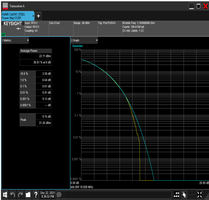
n66_10MHz_15kHz_1745MHz_CP-OFDM 16 QAM_RB52@0
