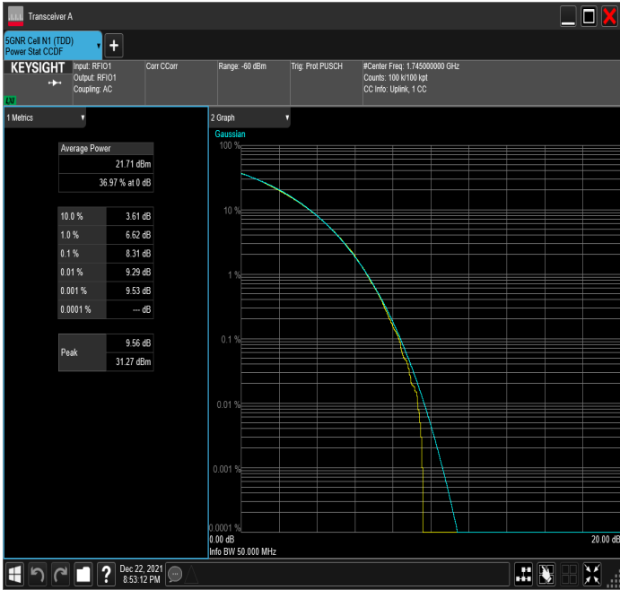
n66_40MHz_15kHz_1745MHz_CP-OFDM 64 QAM_RB216@0
