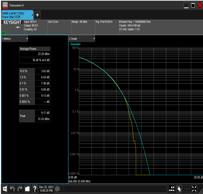
n66_25MHz_15kHz_1745MHz_CP-OFDM QPSK_RB128@0
