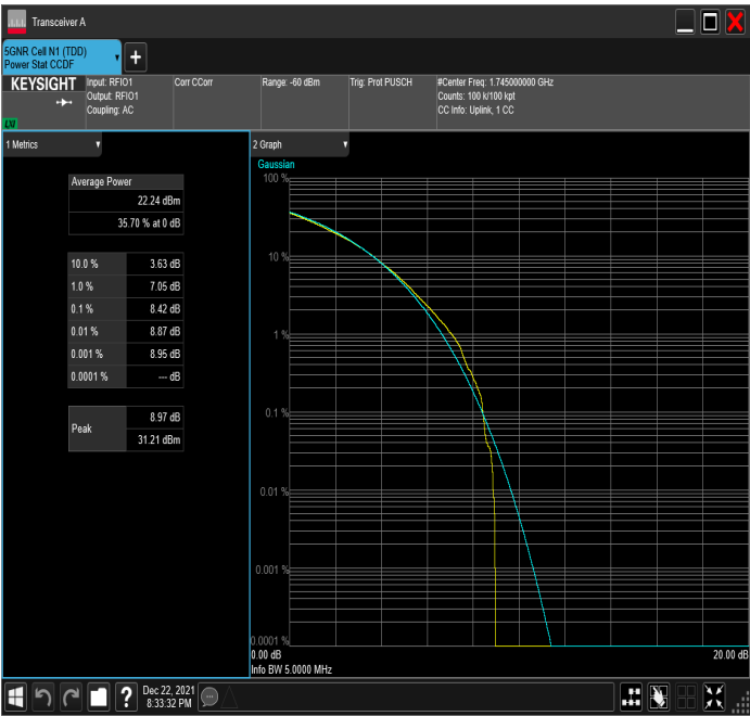
n66_5MHz_15kHz_1745MHz_CP-OFDM 16 QAM_RB25@0
