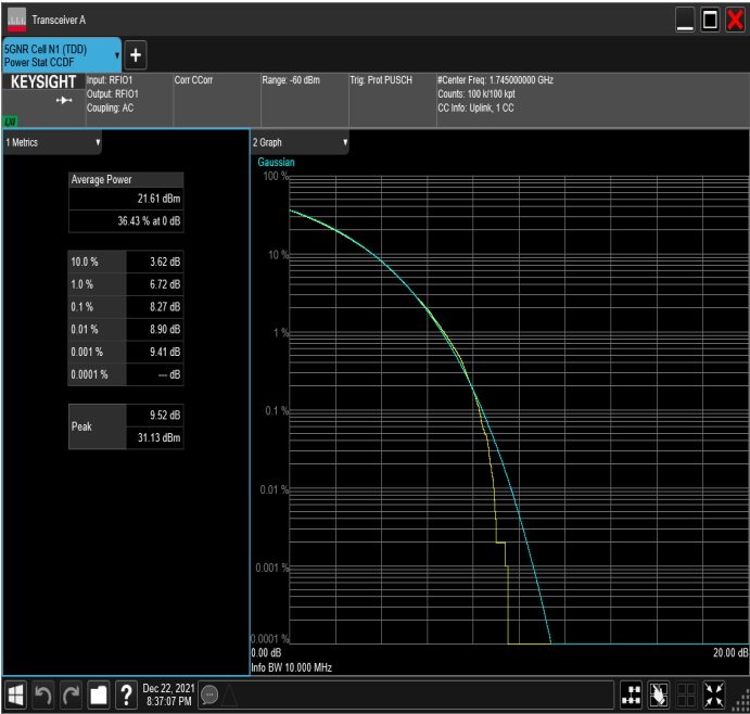
n66_10MHz_15kHz_1745MHz_CP-OFDM 64 QAM_RB52@0
