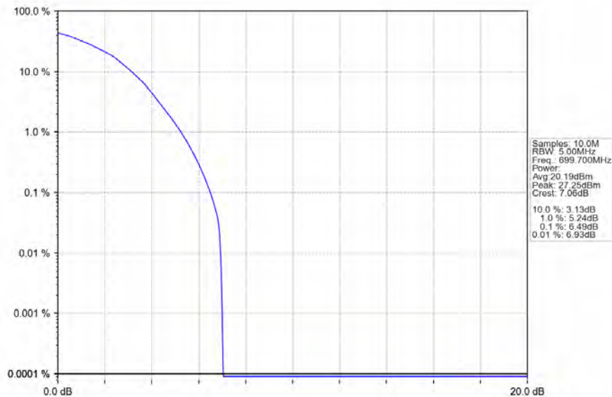
Band12_1.4MHz_64QAM_LCH_699.7MHz_RB_6_0_NTNV
