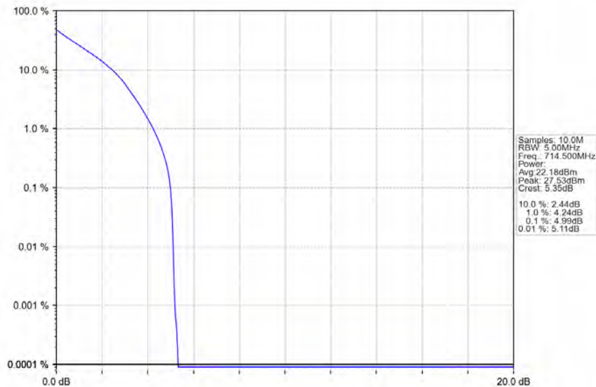
Band12_3MHz_QPSK_HCH_714.5MHz_RB_15_0_NTNV
