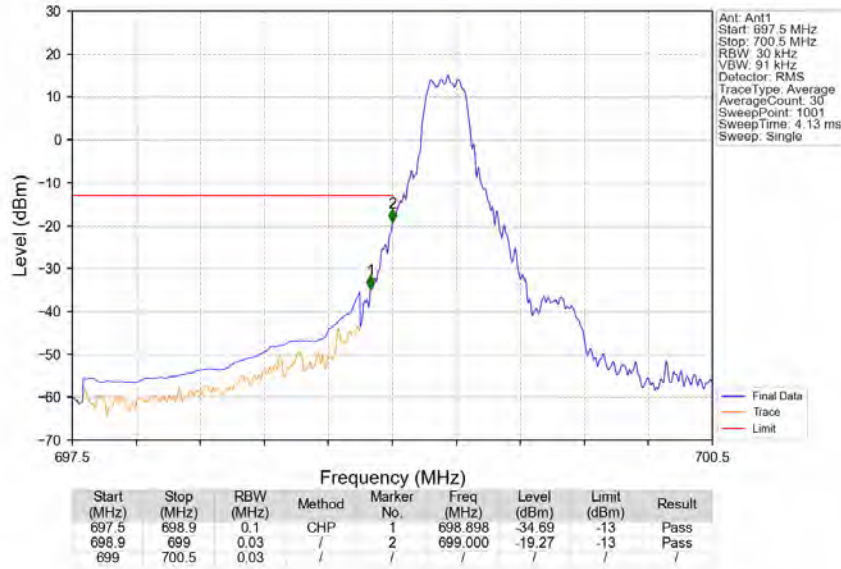
Band12_1.4MHz_64QAM_LCH_699.7MHz_RB_1_0_NTNV
