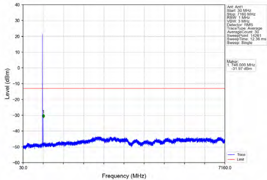
Band12_3MHz_QPSK_HCH_714.5MHz_RB_1_14_NTNV
