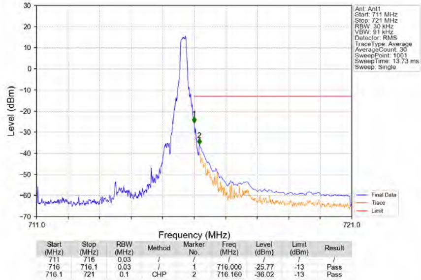
Band12_5MHz_16QAM_HCH_713.5MHz_RB_1_24_NTNV
