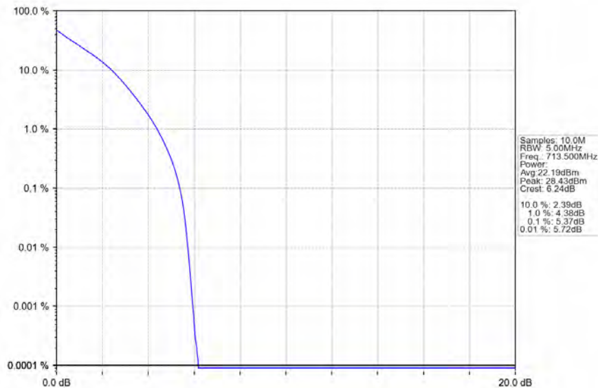
Band12_5MHz_QPSK_HCH_713.5MHz_RB_25_0_NTNV
