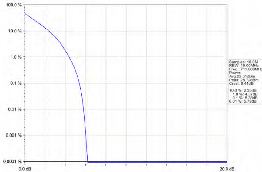
Band12_10MHz_QPSK_HCH_711MHz_RB_50_0_NTNV
