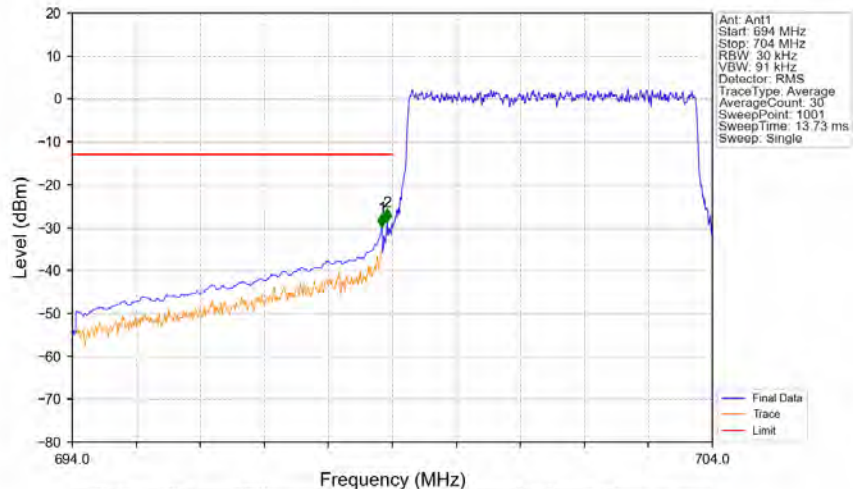
Band12_5MHz_QPSK_LCH_701.5MHz_RB_25_0_NTNV
