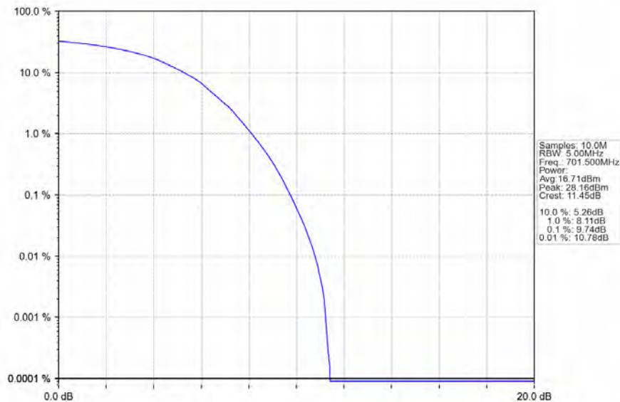
Band12_5MHz_64QAM_LCH_701.5MHz_RB_25_0_NTNV
