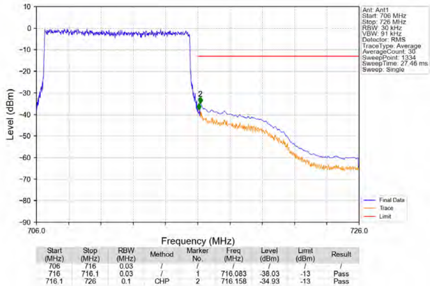
Band12_10MHz_QPSK_HCH_711MHz_RB_50_0_NTNV
