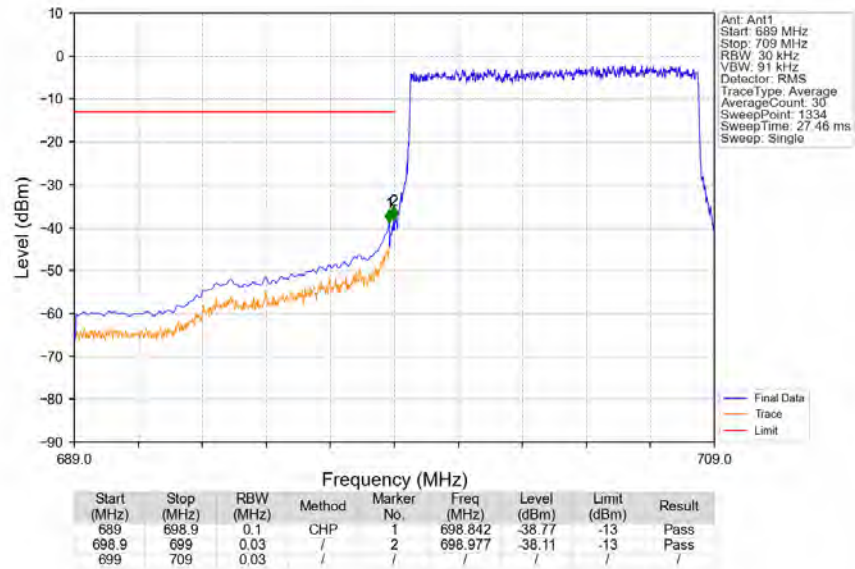
Band12_10MHz_64QAM_LCH_704MHz_RB_50_0_NTNV
