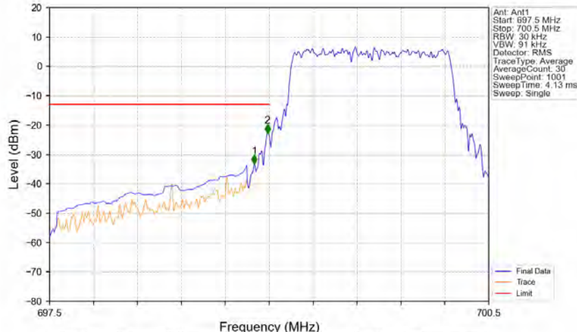
Band12_1.4MHz_64QAM_LCH_699.7MHz_RB_6_0_NTNV
