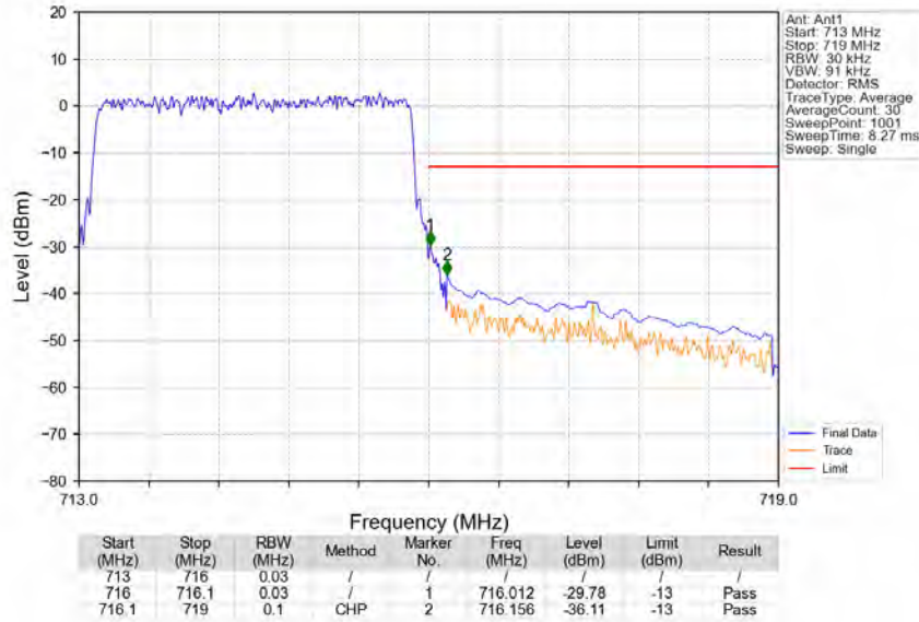
Band12_3MHz_64QAM_HCH_714.5MHz_RB_15_0_NTNV
