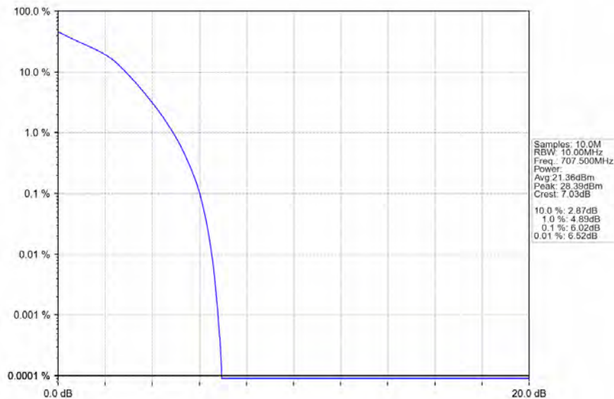
Band12_10MHz_16QAM_MCH_707.5MHz_RB_50_0_NTNV
