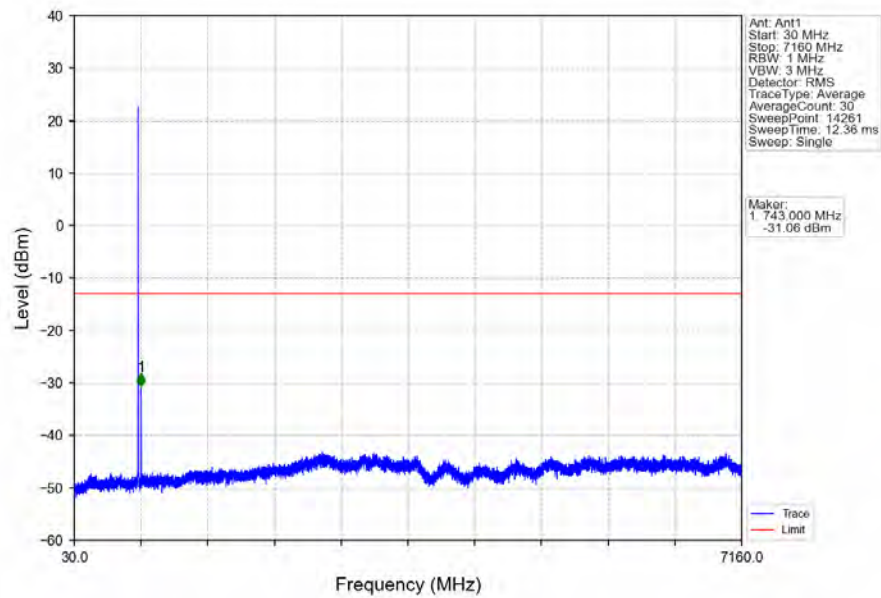
Band12_5MHz_QPSK_HCH_713.5MHz_RB_1_24_NTNV
