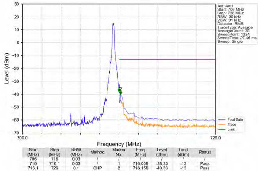
Band12_10MHz_16QAM_HCH_711MHz_RB_1_49_NTNV
