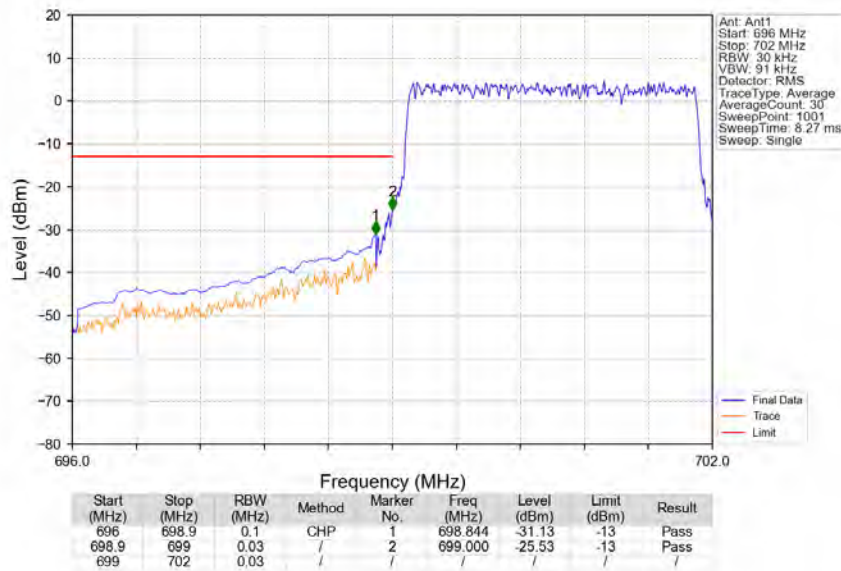
Band12_3MHz_QPSK_LCH_700.5MHz_RB_15_0_NTNV
