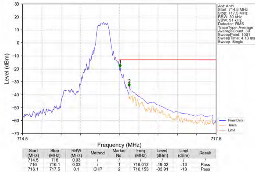
Band12_1.4MHz_16QAM_HCH_715.3MHz_RB_1_5_NTNV
