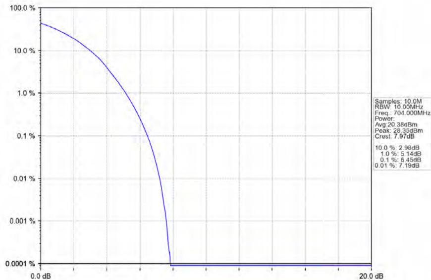
Band12_10MHz_64QAM_LCH_704MHz_RB_50_0_NTNV
