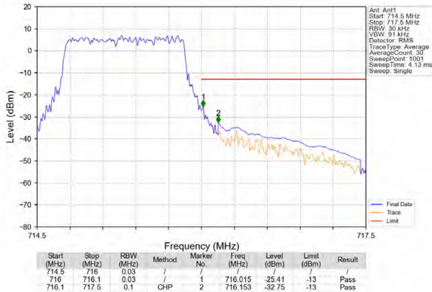
Band12_1.4MHz_64QAM_HCH_715.3MHz_RB_6_0_NTNV
