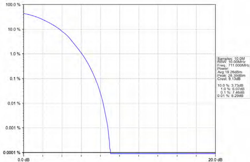
Band12_10MHz_64QAM_HCH_711MHz_RB_50_0_NTNV
