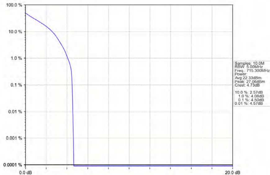
Band12_1.4MHz_QPSK_HCH_715.3MHz_RB_6_0_NTNV
