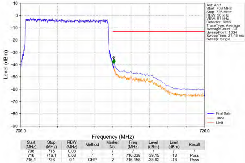
Band12_10MHz_64QAM_HCH_711MHz_RB_50_0_NTNV
