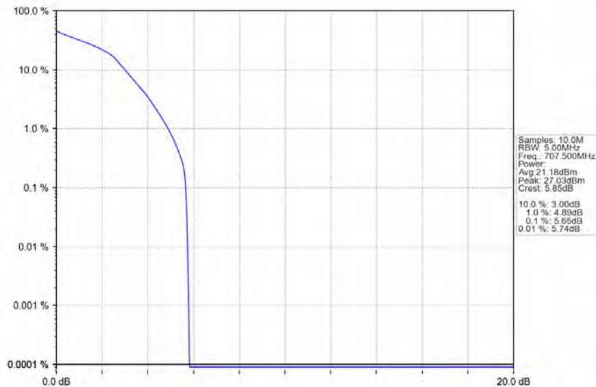
Band12_1.4MHz_16QAM_MCH_707.5MHz_RB_6_0_NTNV
