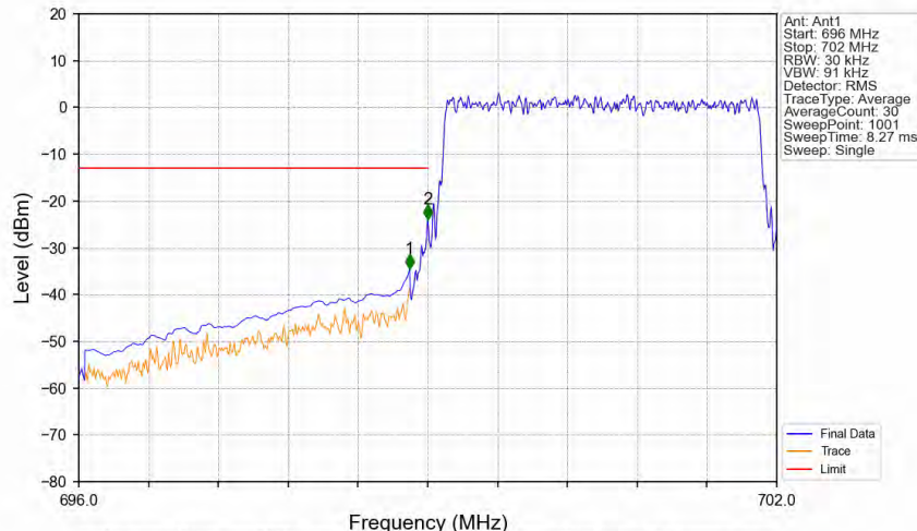
Band12_3MHz_64QAM_LCH_700.5MHz_RB_15_0_NTNV
