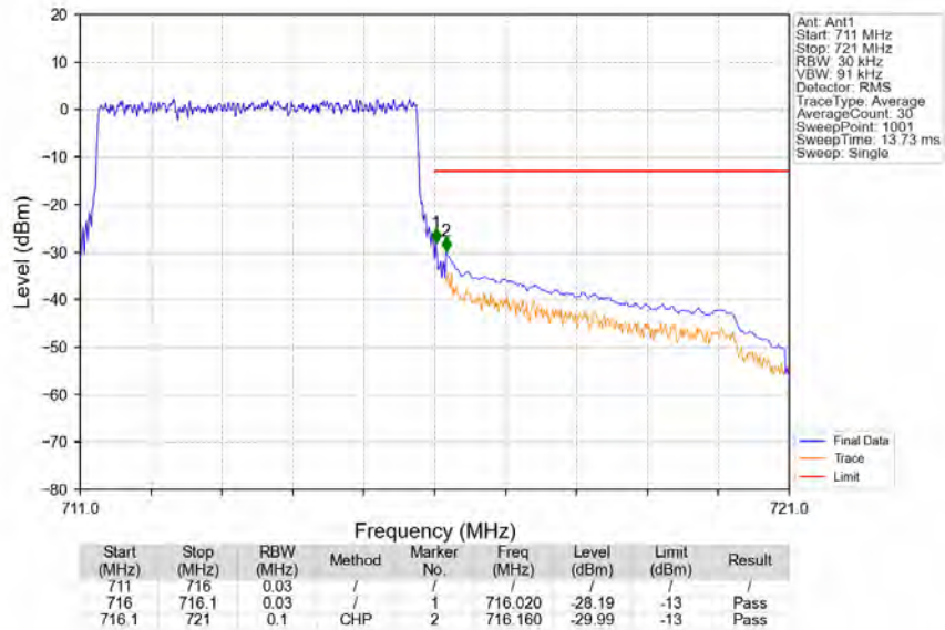
Band12_5MHz_QPSK_HCH_713.5MHz_RB_25_0_NTNV
