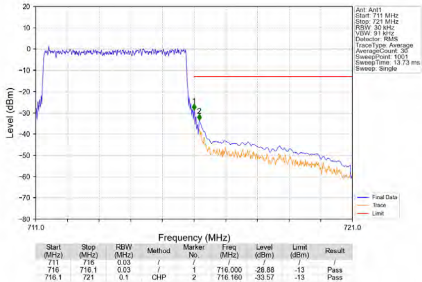
Band12_5MHz_64QAM_HCH_713.5MHz_RB_25_0_NTNV
