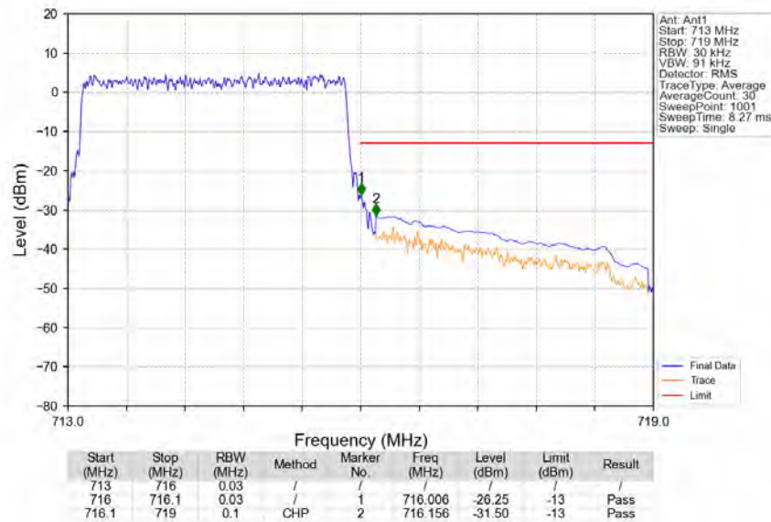
Band12_3MHz_QPSK_HCH_714.5MHz_RB_15_0_NTNV
