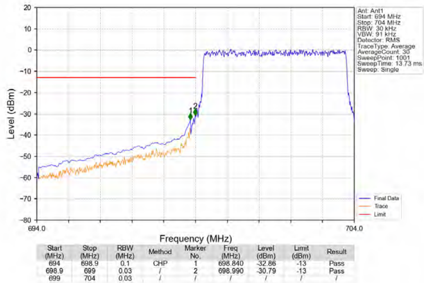
Band12_5MHz_64QAM_LCH_701.5MHz_RB_25_0_NTNV
