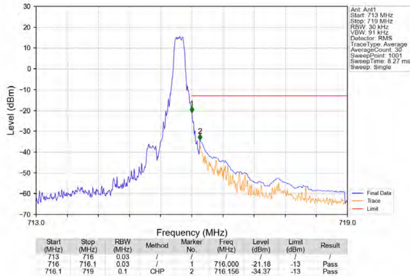
Band12_3MHz_16QAM_HCH_714.5MHz_RB_1_14_NTNV
