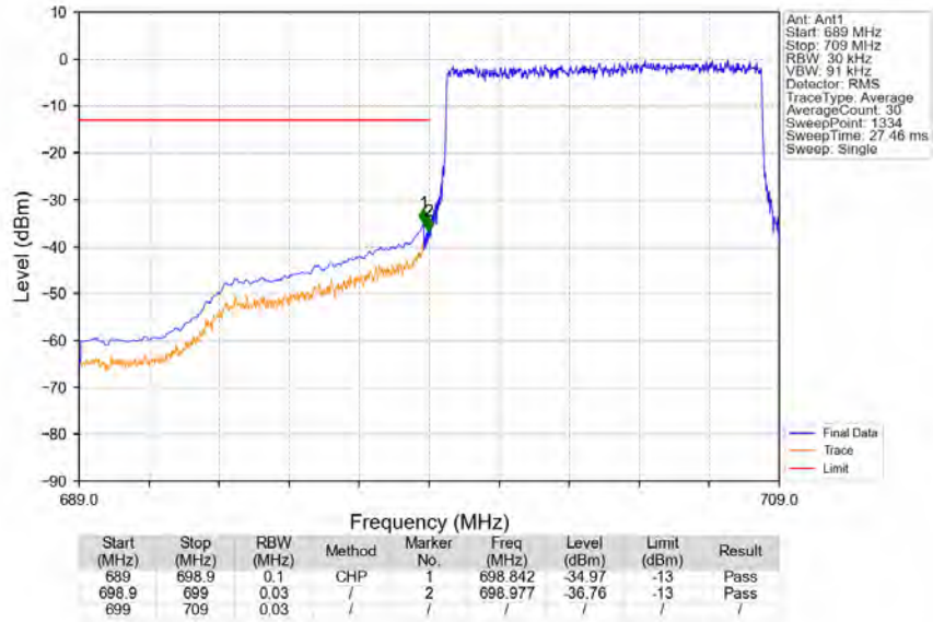
Band12_10MHz_QPSK_LCH_704MHz_RB_50_0_NTNV
