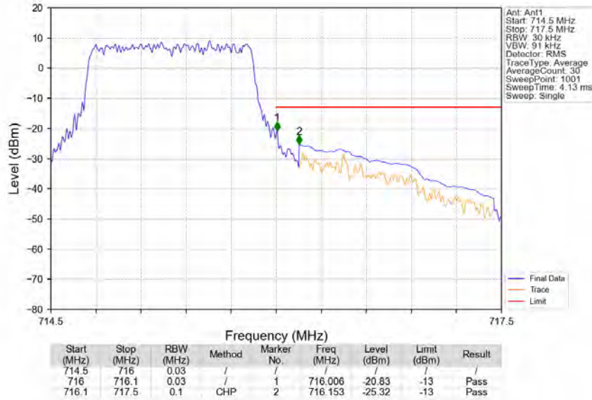
Band12_1.4MHz_QPSK_HCH_715.3MHz_RB_6_0_NTNV
