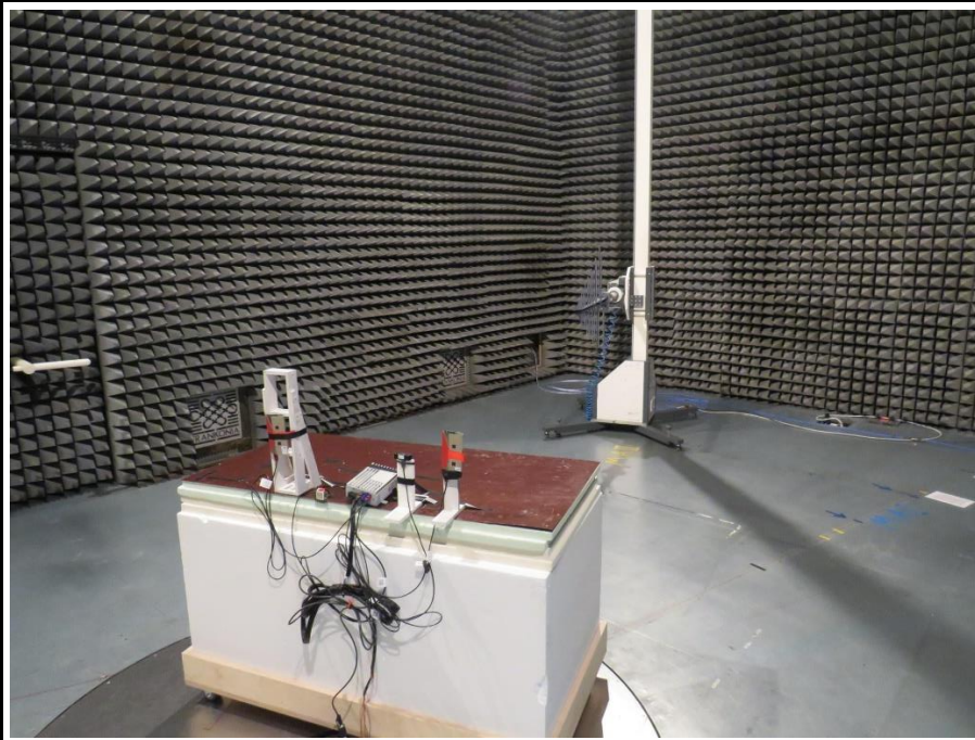
Test setup 200 to 1000 MHz
