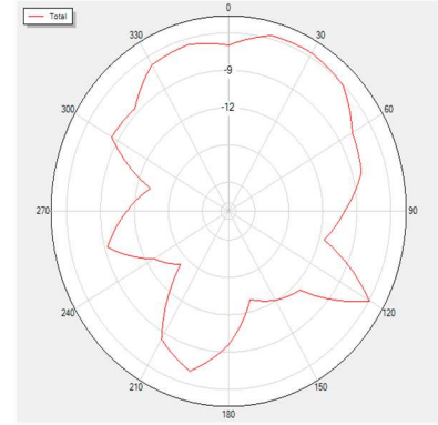
2500P90 Total
