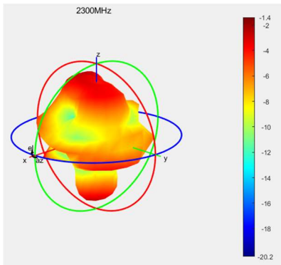
2300P0 Total
