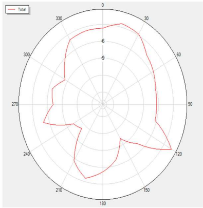
2450P90 Total
