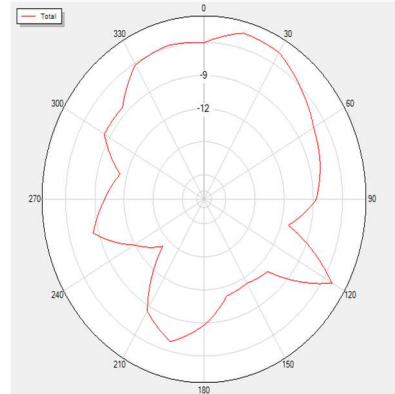
2500P90 Total
