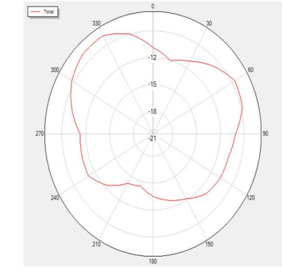
2500T90 Total
