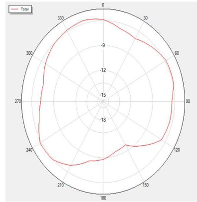
2450T90 Total
