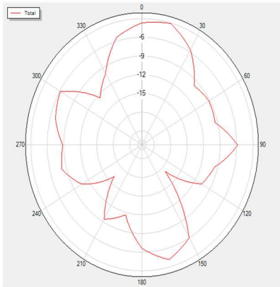
2450P0 Total
