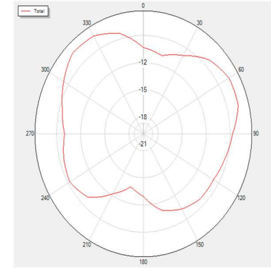
2500T90 Total
