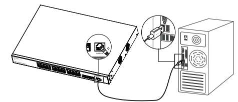
Connect to Console Port (USB)
