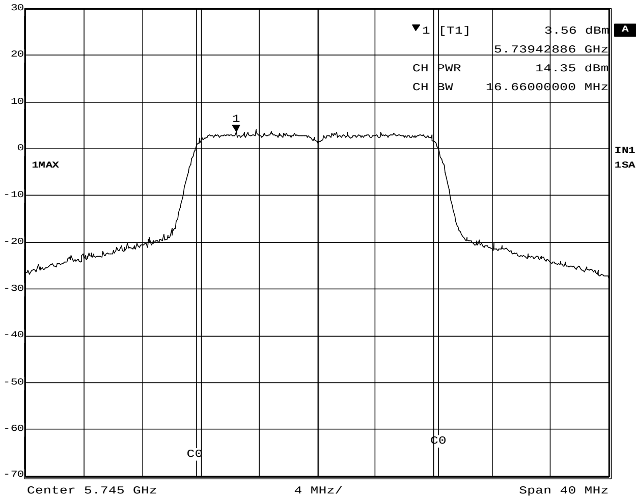
Plot 3-4. Conducted Peak Output Power of 5745MHz
