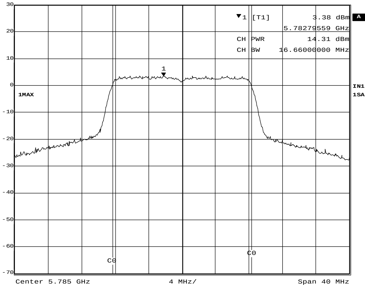
Plot 3-5. Conducted Peak Output Power of 5785MHz
