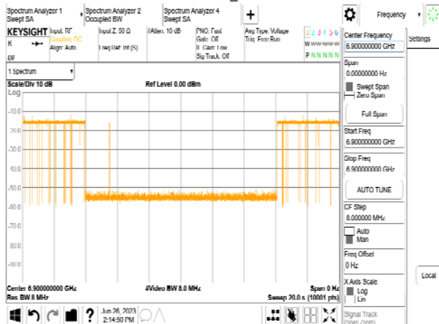
802.11be_320MHz_CF 6745MHz_Interference_6900MHz_ -79.32dBm_Normal
