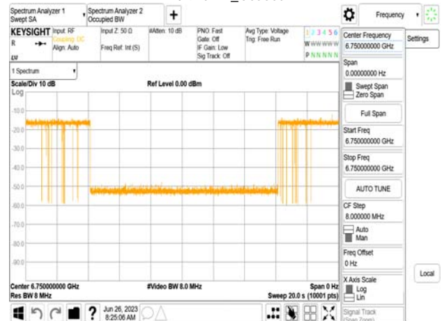
802.11be_320MHz_CF 6905MHz_Interference_6750MHz_ -76.92dBm_Minimal
