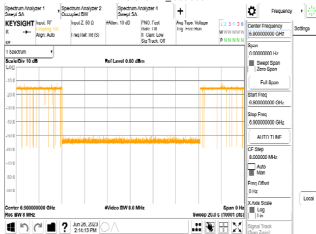
802.11be_320MHz_CF 6745MHz_Interference_6900MHz_ -75.32dBm_Minimal
