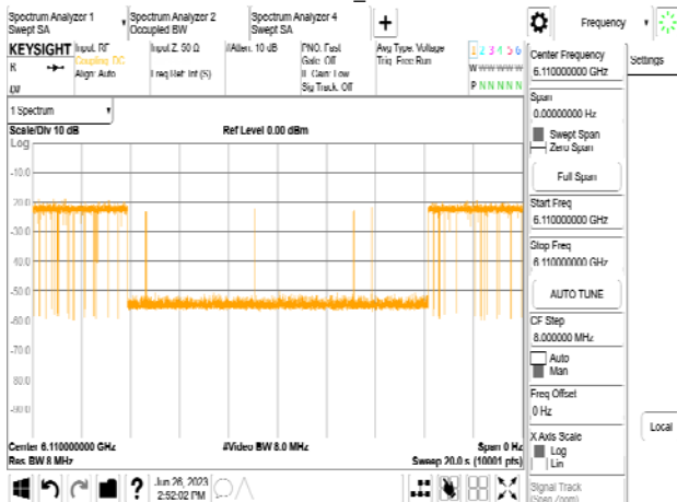
802.11be_320MHz_CF 6265MHz_Interference_6110MHz_ -76.48dBm_Normal
