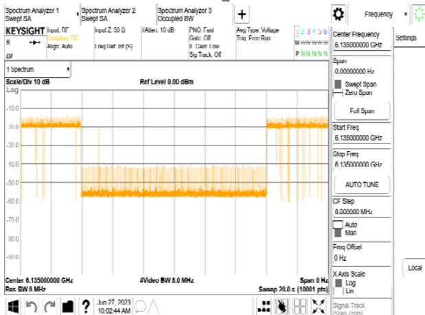
802.11be_20MHz_CF 6135MHz_Interference_6135MHz_-82.25dBm_Normal
