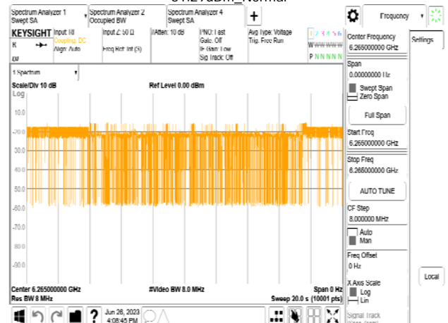
802.11be_320MHz_CF 6265MHz_Interference_6265MHz_ -81.29dBm_Normal
