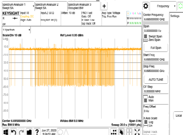
802.11be_20MHz_CF 6695MHz_Interference_6695MHz_-83.47dBm_Normal
