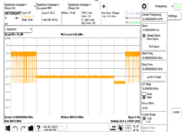
802.11be_320MHz_CF 6265MHz_Interference_6265MHz_ -70.29dBm_Minimal
