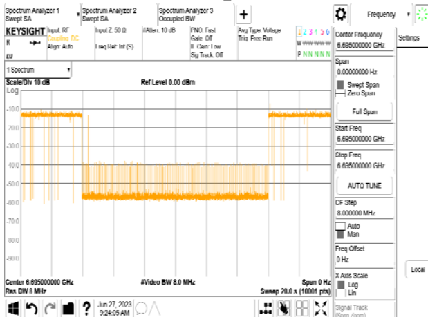
802.11be_20MHz_CF 6695MHz_Interference_6695MHz_-83.47dBm_Normal
