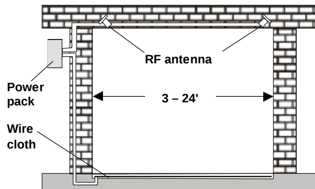
Figure 2. Concealed antennas with wire cloth
